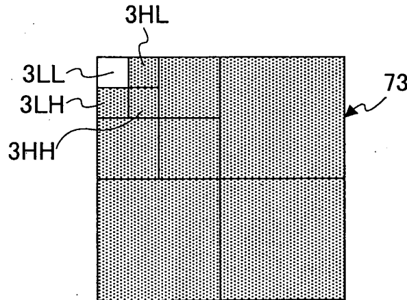
DECOMPOSITION_LEVEL_3
