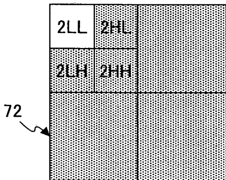
DECOMPOSITION_LEVEL_2
