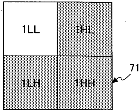
DECOMPOSITION_LEVEL_1
