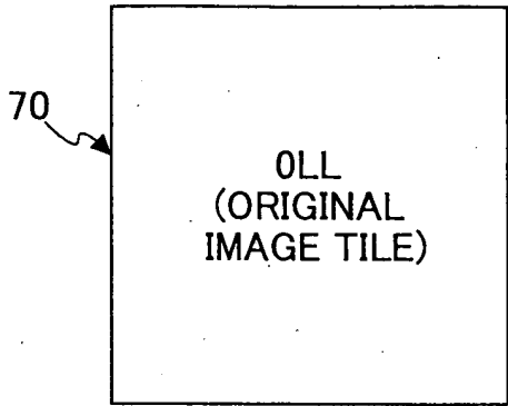
DECOMPOSITION_LEVEL_0
