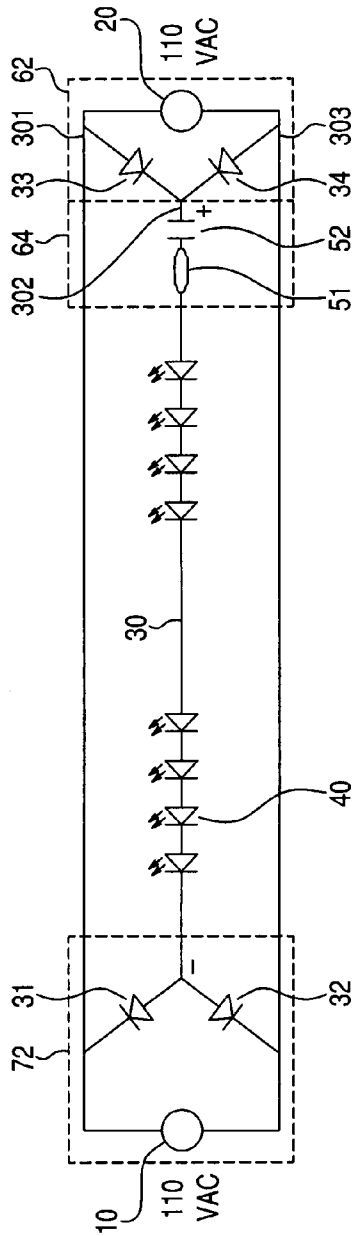
Fig. 3 Prior Art
