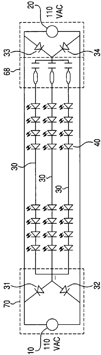
Fig. 4 Prior Art
