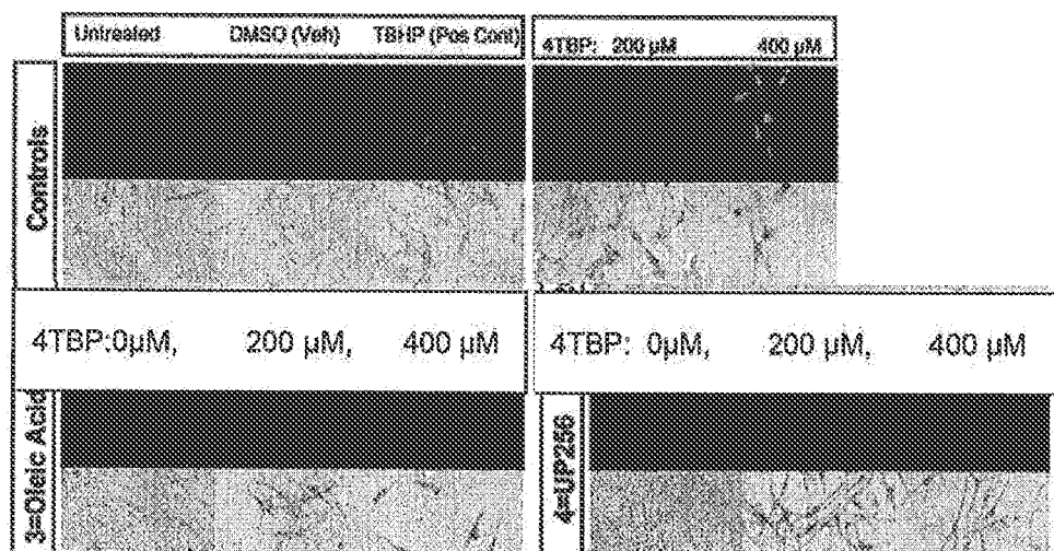
Figure 3. Protection from ROS. Cells were plated and treated with test compounds alone and with 4-TBP at two concentrations to assess the protective properties of the test compounds against 4-TBP induced ROS. As a positive control, TBHP, an activated form of H 2 O 2 as well as 4-TBP treatment in a dose dependent manner was used. Treatment induced fluorescence indicating ROS presence. UP256 ameliorated the effects of the treatment with 4-TBP while sustaining viability.
