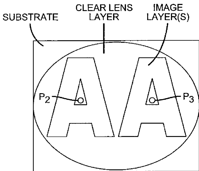
TOP VIEW (ELLIPTICAL LENS ON TWO LETTERS)
