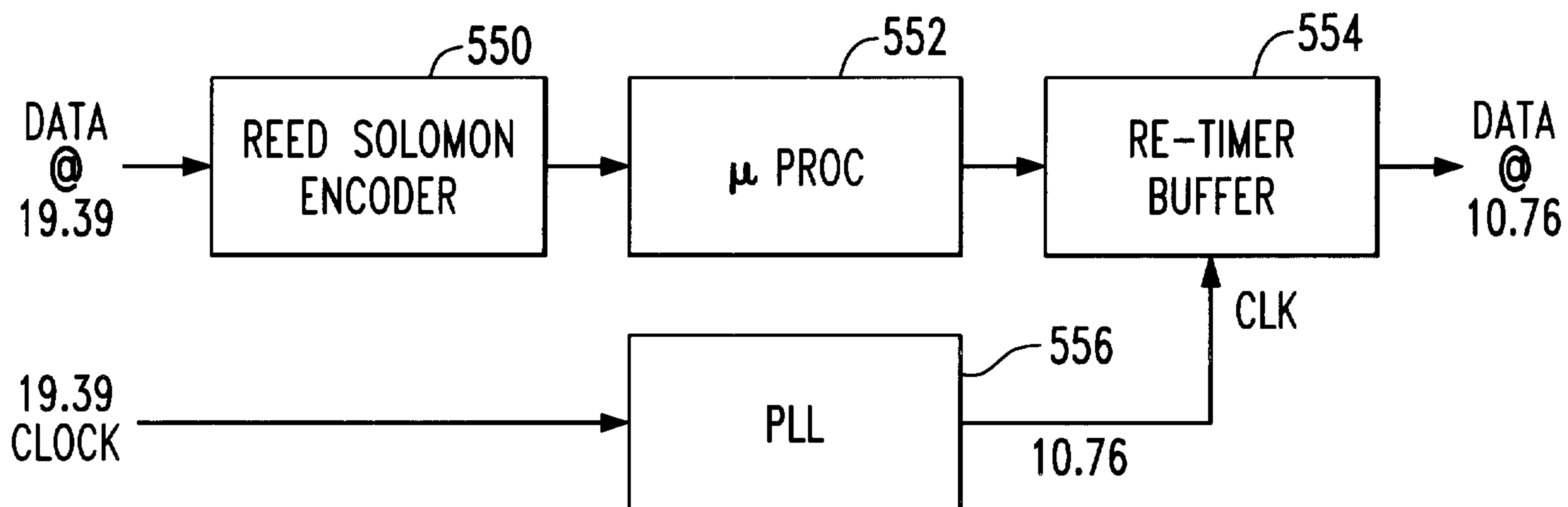
FIG. 6 PRIOR ART
