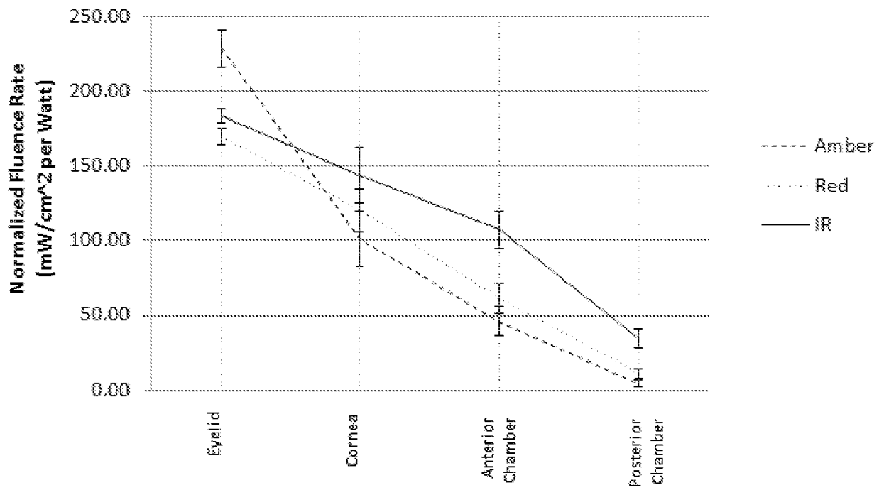
Mean ± SEM Fluence Rate, All Subjects, Closed Eye Normalized to 1W Device Output
