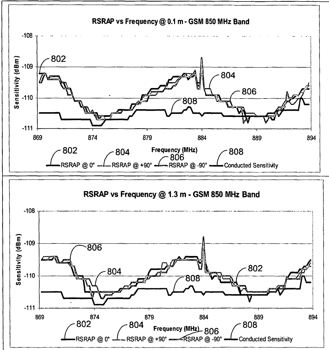
FIG. 8a - RSRAP for different azimuth angles and distances to wireless device under test and conducted sensitivity - GSM 850 MHz Band.
