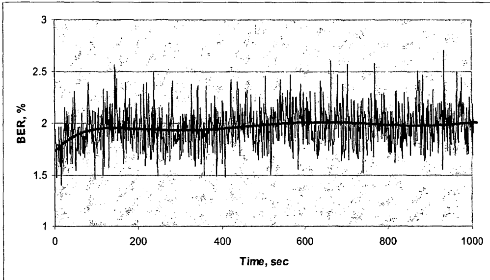
FIG. 6 - BER vs. time
