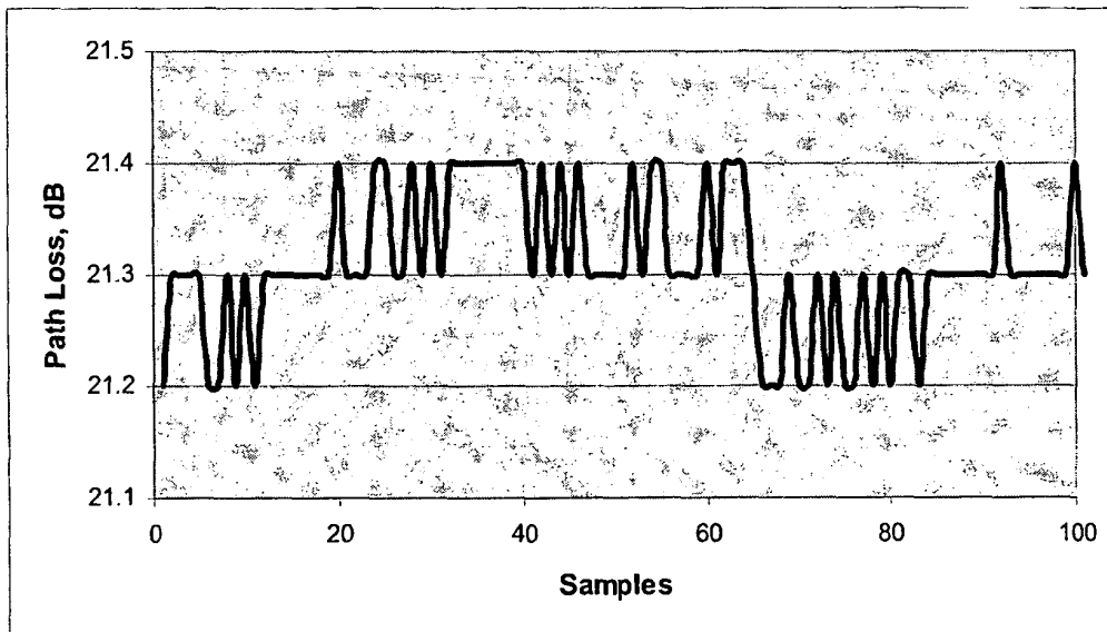
FIG. 7 - Path loss variation
