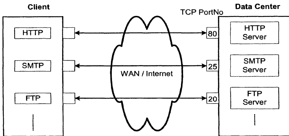
Well-Known TCP port (Softport) Connections
