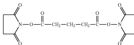
DSG (Disuccinimidyl Glutarate) MW 326.26 Spacer Arm Length 7.72A
