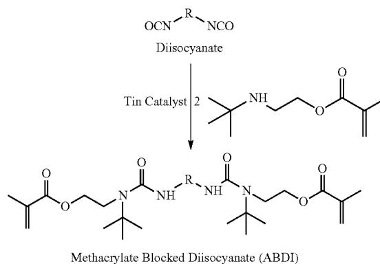
Methacrylate Blocked Diisocyanate (ABDI)
