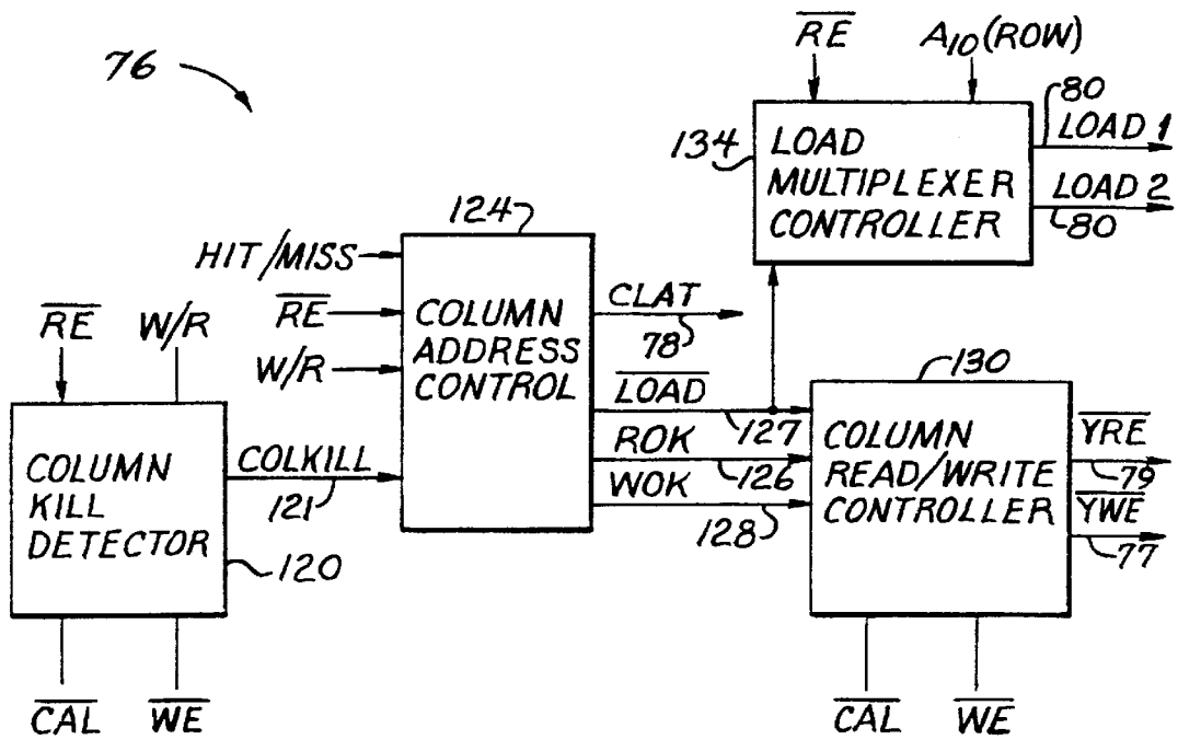
COLUMN ADDRESS CONTROL LOGIC
