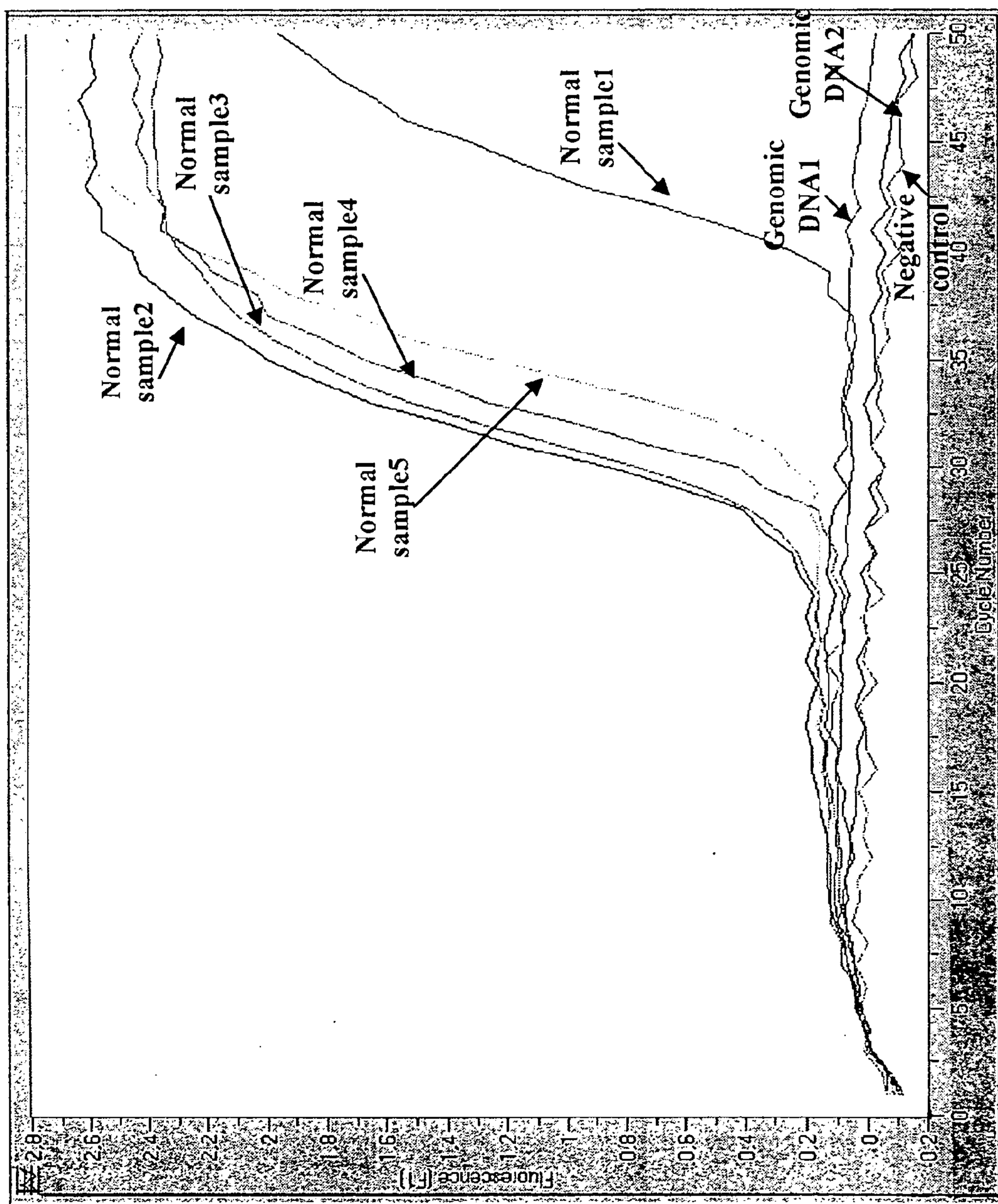
Figure 4 A typical real-time PCR graph for PBGD
