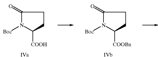
SCHEME IV
