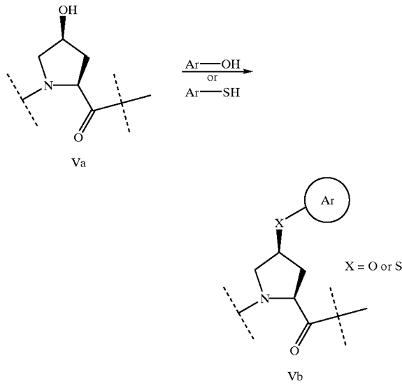
SCHEME V
