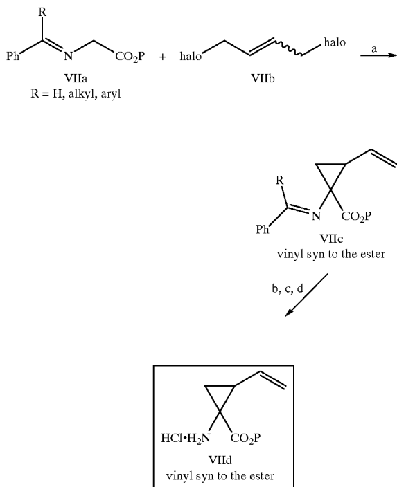
SCHEME VII
