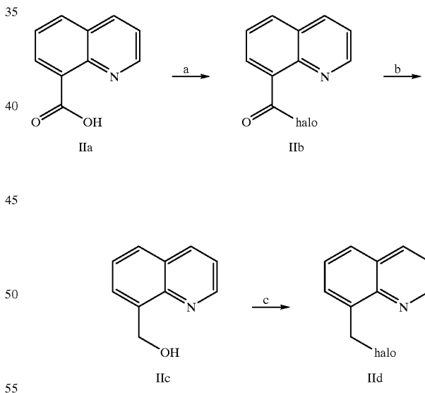
SCHEME II
