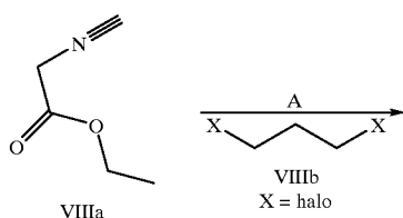
SCHEME VIII
