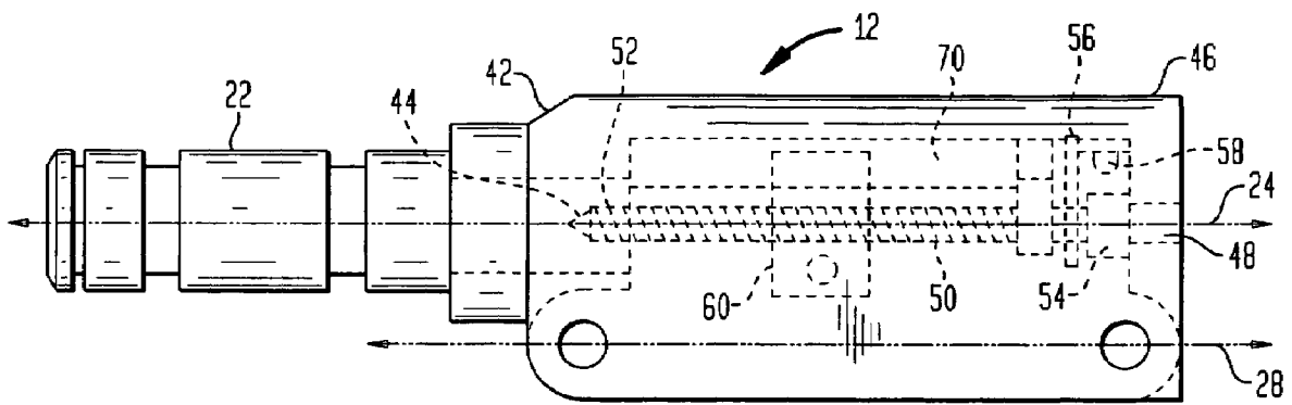
FIG. 2 (PRIOR ART)
