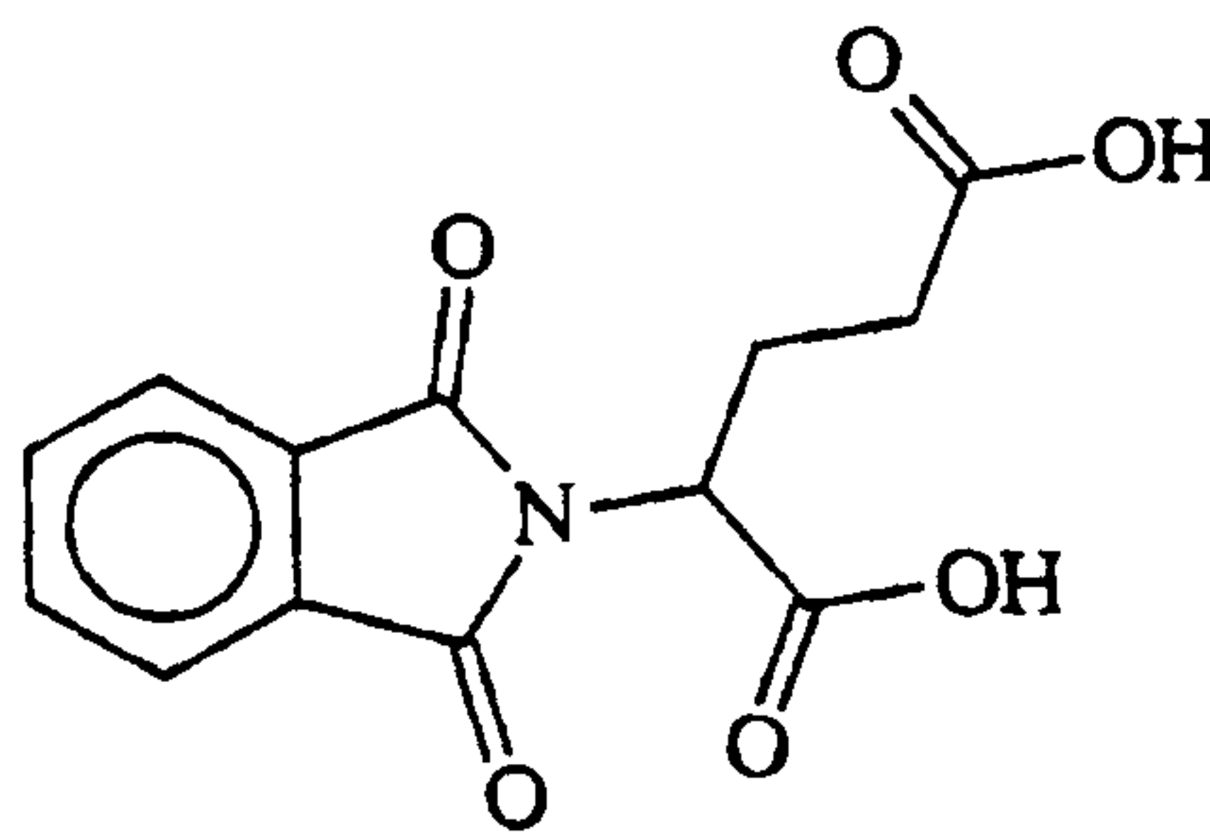
phthaloyl glutamic acid (PG Acid)
