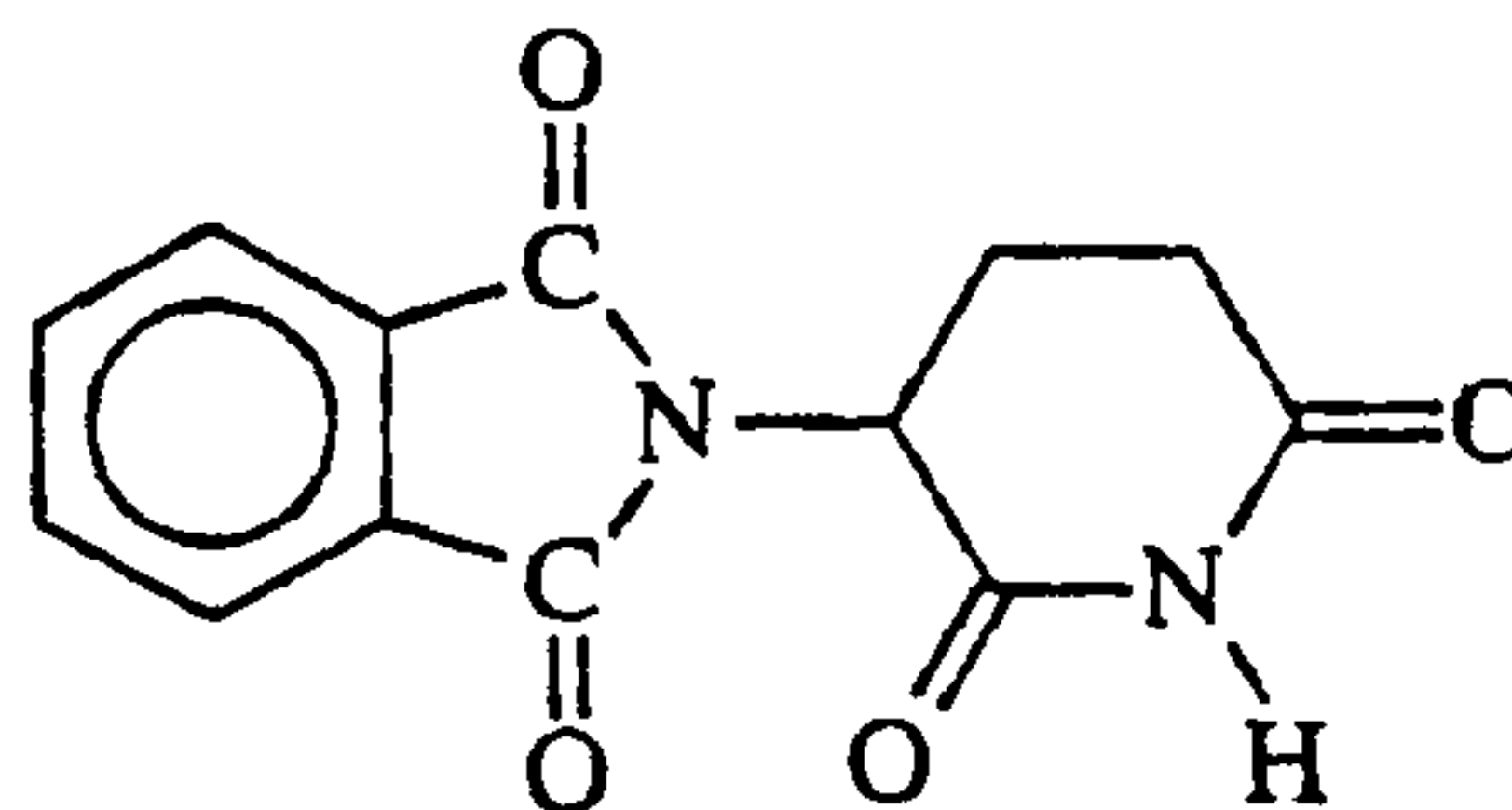
thalidomide
