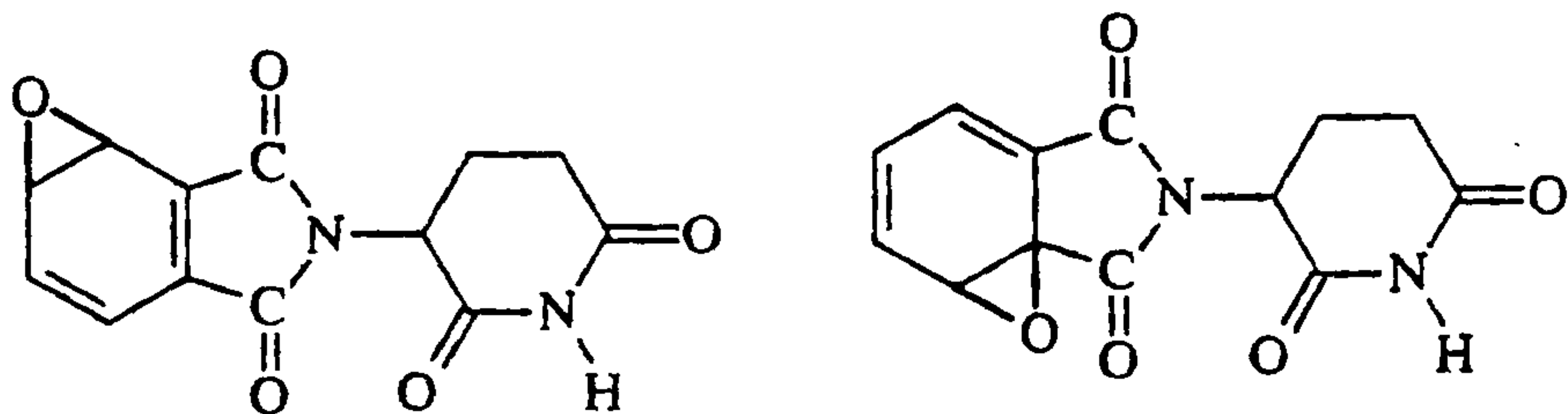
Epoxides of thalidomide
