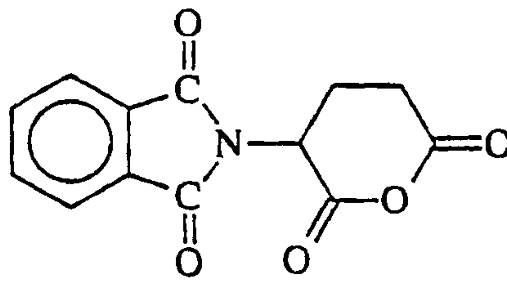
phthaloyl glutamic anhydride (PGA)
