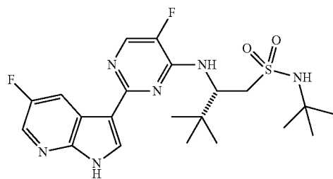
(S)-2-(5-Fluoro-2-(5-fluoro-1H-pyrrolo[2,3-b]pyridin-3-yl)pyrimidin-4-ylamino)-N-tert-butyl-3,3-dimethyl-N-propylbutane-1-sulfonamide (40)
