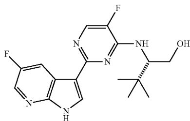
(S)-2-(5-fluoro-2-(5-fluoro-1H-pyrrolo[2,3-b]pyridin-3-yl)pyrimidin-4-ylamino)-3,3-dimethylbutane-1-ol (32)
