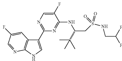
(S)-N-(2,2-difluoroethyl)-2-(5-fluoro-2-(5-fluoro-1H-pyrrolo[2,3-b]pyridin-3-yl)pyrimidin-4-ylamino)-3,3-dimethylbutane-1-sulfonamide (57)
