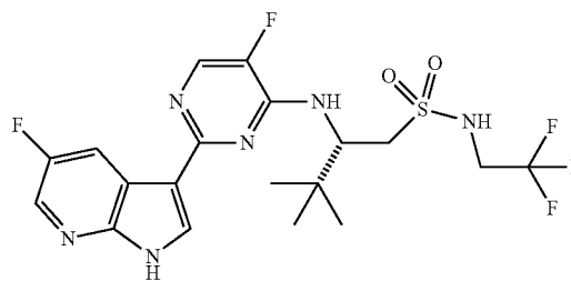
(S)-2-(5-fluoro-2-(5-fluoro-1H-pyrrolo[2,3-b]pyridin-3-yl)pyrimidin-4-ylamino)-3,3-dimethyl-N-(2,2,2-trifluoroethyl)butane-1-sulfonamide (58)
