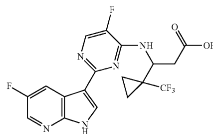
(+/-)-3-((5-Fluoro-2-(5-fluoro-1H-pyrrolo[2,3-b]pyridin-3-yl)pyrimidin-4-ylamino)-3-(1-(trifluoroethyl)cyclopropyl)propanoic acid (93)
