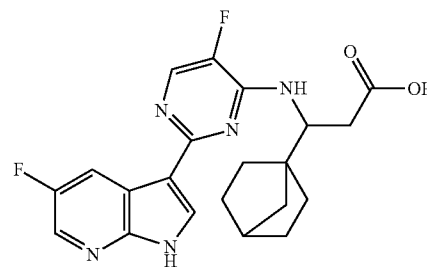
(+/-)-3-(Bicyclo[2.2.1]heptan-1-yl)-3-(5-fluoro-2-(5-fluoro-1H-pyrrolo[2,3-b]pyridin-3-yl)pyrimidin-4-ylamino)propanoic acid (95)
