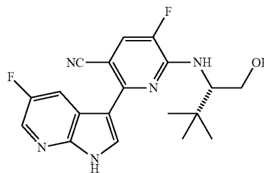
(S)-5-fluoro-2-((5-fluoro-1H-pyrrolo[2,3-b]pyridin-3-yl)-6-((1-hydroxy-3,3-dimethylbutan-2-yl)amino)nicotinonitrile (24)
