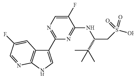
(S)-2-(5-fluoro-2-(5-fluoro-1H-pyrrolo[2,3-b]pyridin-3-yl)pyrimidin-4-ylamino)-3,3-dimethylbutane-1-sulfonic acid (11)
