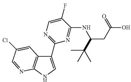
(S)-3-((2-(5-chloro-1H-pyrrolo[2,3-b]pyridin-3-yl)-5-fluoropyrimidin-4-yl)amino)-4,4-dimethylpentanoic acid (3)
