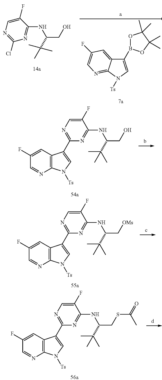
Synthetic Scheme 10
