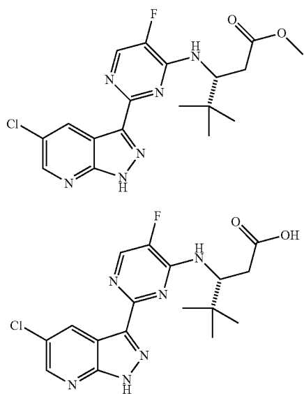
(R)-3-((2-(5-chloro-1H-pyrazolo[3,4-b]pyridin-3-yl)-5-fluoropyrimidin-4-yl)amino)-4,4-dimethylpentanoic acid (97) and methylester (96)
