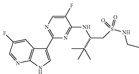
(S)-N-Ethyl-2-(5-fluoro-2-(5-fluoro-1H-pyrrolo[2,3-b]pyridin-3-yl)pyrimidin-4-ylamino)-3,3-dimethylbutane-1-sulfonamide (33)
