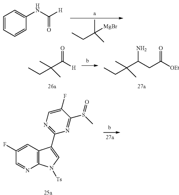
Synthetic Scheme 5
