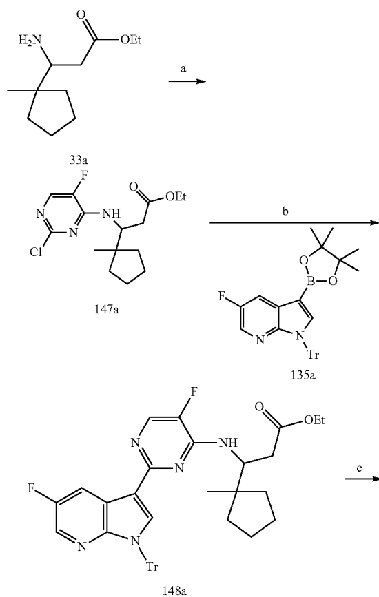
Synthetic Scheme 22
