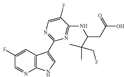
(+/-)-5-Fluoro-3-((5-fluoro-2-(5-fluoro-1H-pyrrolo[2,3-b]pyridin-3-yl)pyrimidin-4-ylamino)-4,4-dimethylpentanoic acid (76)
