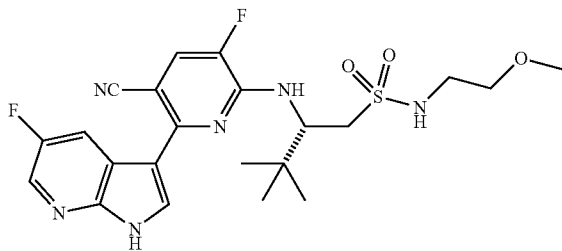
(S)-2-((5-cyano-3-fluoro-6-(5-fluoro-1H-pyrrolo[2,3-b]pyridin-3-yl)pyridin-2-ylamino)-N-(2-methoxyethyl)-3,3-dimethylbutane-1-sulfonamide (29)
