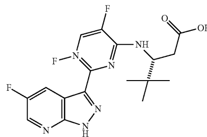
(R)-3-((3,5-difluoro-6-(5-fluoro-1H-pyrazolo[3,4-b]pyridin-3-yl)pyrimidin-2-yl)amino)-4,4-dimethylpentanoic acid (6)
