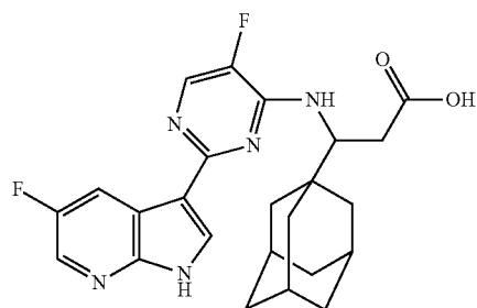
(+/-)-3-(1-Adamantyl)-3-[[5-fluoro-2-(5-fluoro-1H-pyrrolo[2,3-b]pyridin-3-yl)pyrimidin-4-yl]amino]propionic acid (86)
