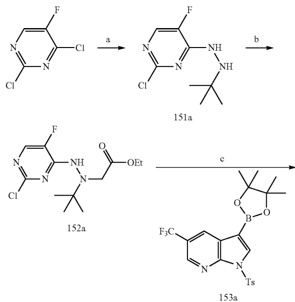
Synthetic Scheme 23
