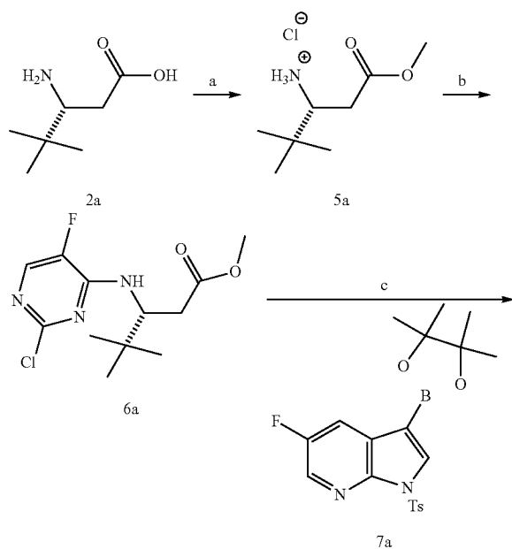
Synthetic Scheme 2
