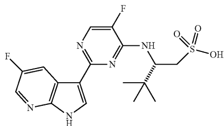
(S)-2-((5-fluoro-2-(5-fluoro-1H-pyrrolo[2,3-b]pyridin-3-yl)pyrimidin-4-yl)amino)-3,3-dimethylbutane-1-sulfonic acid (11)
