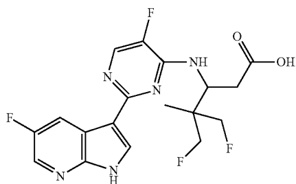
(+/-)-5-Fluoro-3-((5-fluoro-2-(5-fluoro-1H-pyrrolo[2,3-b]pyridin-3-yl)pyrimidin-4-yl)amino)-4-(fluoromethyl)-4-methylpentanoic acid (84)
