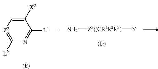
General Scheme 1
