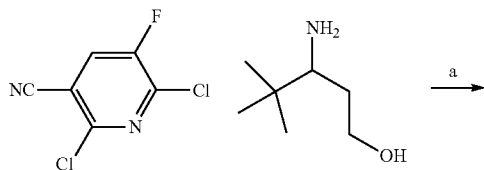
Synthetic Scheme 15
