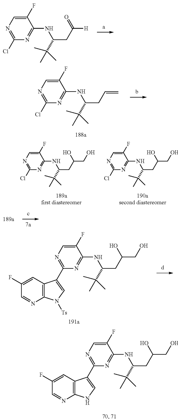
Synthetic Scheme 30
