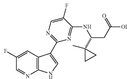
(R)-3-((5-fluoro-2-(5-fluoro-1H-pyrrolo[2,3-b]pyridin-3-yl)pyrimidin-4-ylamino)-3-(1-methylcyclopropyl)propanoic acid (91)
