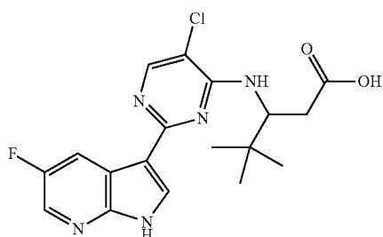
(+/-)-3-((5-chloro-2-(5-fluoro-1H-pyrrolo[2,3-b]pyridin-3-yl)pyrimidin-4-yl)amino)-4,4-dimethylpentanoic acid (85)
