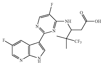
(+/-)-5,5,5-Trifluoro-3-(5-fluoro-2-(5-fluoro-1H-pyrrolo[2,3-b]pyridin-3-yl)pyrimidin-4-ylamino)-4,4-dimethylpentanoic acid (79)
