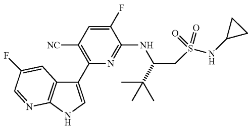
(S)-2-((5-Cyano-3-fluoro-6-(5-fluoro-1H-pyrrolo[2,3-b]pyridin-3-yl)pyridin-2-ylamino)-N-cyclopropyl-3,3-dimethylbutane-1-sulfonamide (28)
