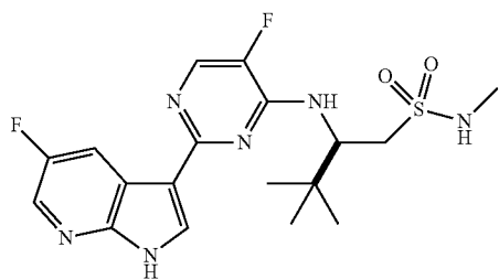
(R)-2-((5-fluoro-2-(5-fluoro-1H-pyrrolo[2,3-b]pyridin-3-yl)pyrimidin-4-yl)amino)-N,3,3-trimethylbutane-1-sulfonamide (38)
