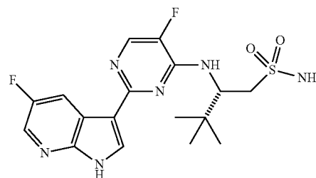
(S)-2-(5-fluoro-2-(5-fluoro-1H-pyrrolo[2,3-b]pyridin-3-yl)pyrimidin-4-ylamino)-3,3-dimethylbutane-1-sulfonamide (22)
