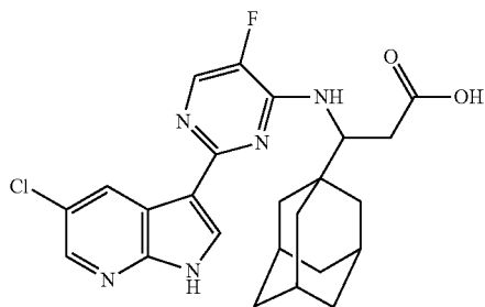
(+/-)-3-(1-Adamantyl)-3-[[2-(5-chloro-1H-pyrrolo[2,3-b]pyridin-3-yl)-5-fluoro-pyrimidin-4-yl]amino]propionic acid (94)
