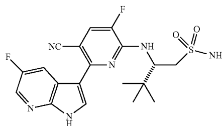
(S)-2-((5-cyano-3-fluoro-6-(5-fluoro-1H-pyrrolo[2,3-b]pyridin-3-yl)pyridin-2-ylamino)-3,3-dimethylbutane-1-sulfonamide (30)
