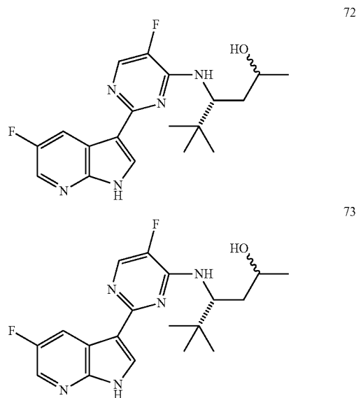
(4R)-4-((5-Fluoro-2-(5-fluoro-1H-pyrrolo[2,3-b]pyridin-3-yl)pyrimidin-4-yl)amino)-5,5-dimethylhexan-2-ol (72 and 73)
