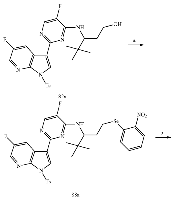
Synthetic Scheme 14
