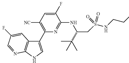
(S)-2-((5-cyano-3-fluoro-6-(5-fluoro-1H-pyrrolo[2,3-b]pyridin-3-yl)pyridin-2-ylamino)-3,3-dimethyl-N-propylbutane-1-sulfonamide (31)
