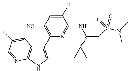
(S)-2-((5-Cyano-3-fluoro-6-(5-fluoro-1H-pyrrolo[2,3-b]pyridin-3-yl)pyridin-2-ylamino)-N,N,3,3-dimethylbutane-1-sulfonamide (27)
