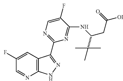
(R)-3-((5-fluoro-2-(5-fluoro-1H-pyrazolo[3,4-b]pyridin-3-yl)pyrimidin-4-yl)amino)-4,4-dimethylpentanoic acid (5)
