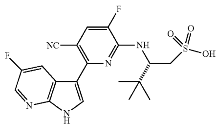
(S)-2-((5-cyano-3-fluoro-6-(5-fluoro-1H-pyrrolo[2,3-b]pyridin-3-yl)pyridin-2-yl)amino)-3,3-dimethylbutane-1-sulfonic acid (25)
