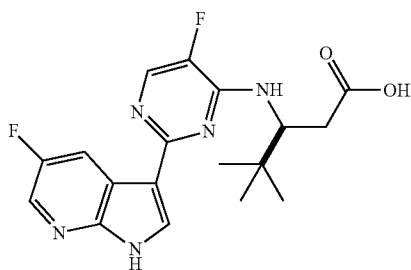
(S)-3-((5-fluoro-2-(5-fluoro-1H-pyrrolo[2,3-b]pyridin-3-yl)pyrimidin-4-yl)amino)-4,4-dimethylpentanoic acid (4)
