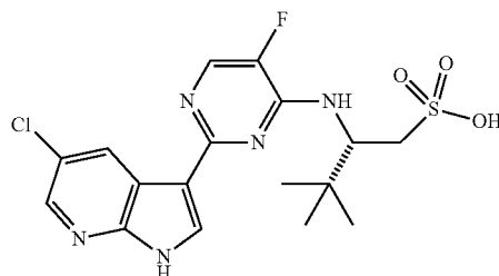
(S)-2-((2-(5-chloro-1H-pyrrolo[2,3-b]pyridin-3-yl)-5-fluoropyrimidin-4-yl)amino)-3,3-dimethylbutane-1-sulfonic acid (10)
