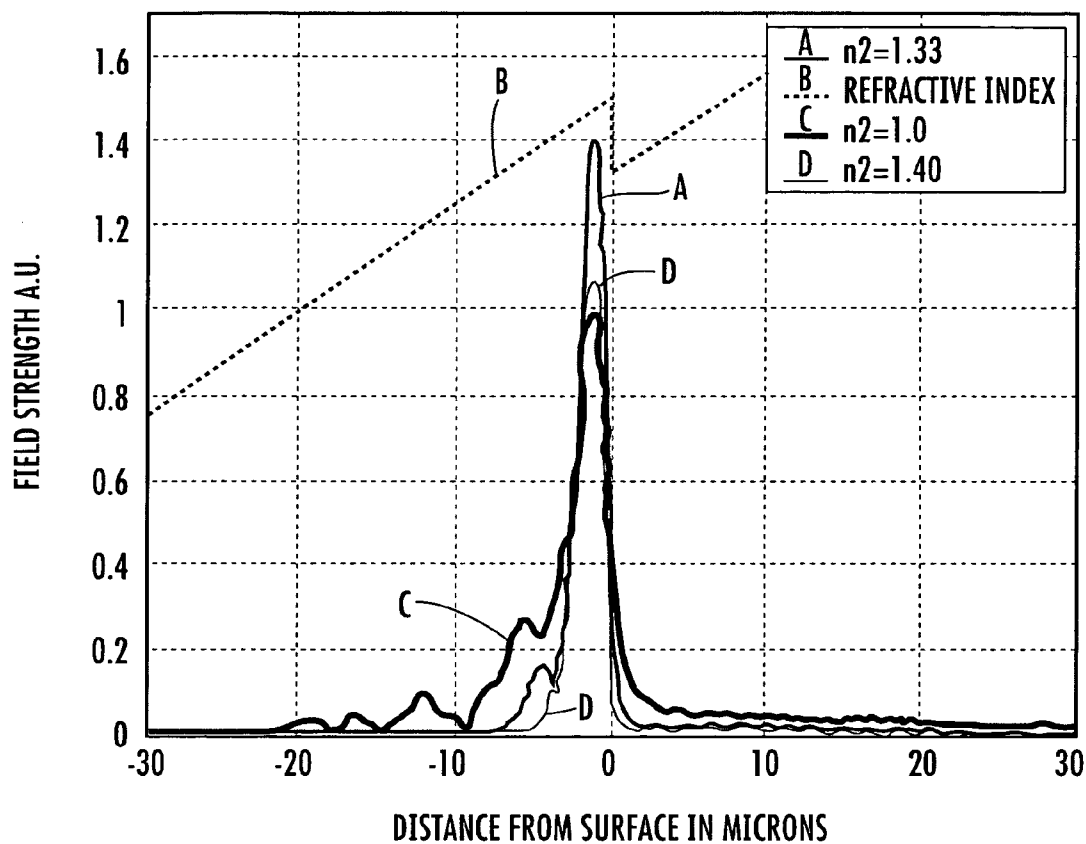
MODELED WHISPERING GALLERY MODE ON A MICROCYLINDER
