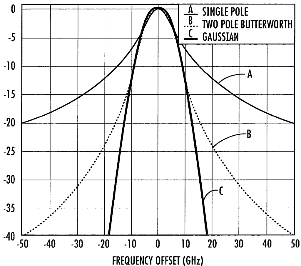
BANDSHAPE FOR GAUSSIAN AND BUTTERWORTH FILTERS
