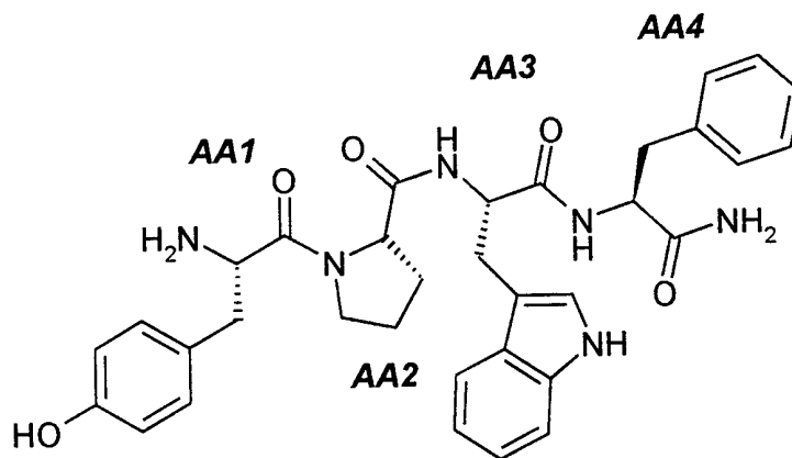
Endomorphin 1 (1) [Tyr-Pro-Trp-Phe-NH 2 ]
