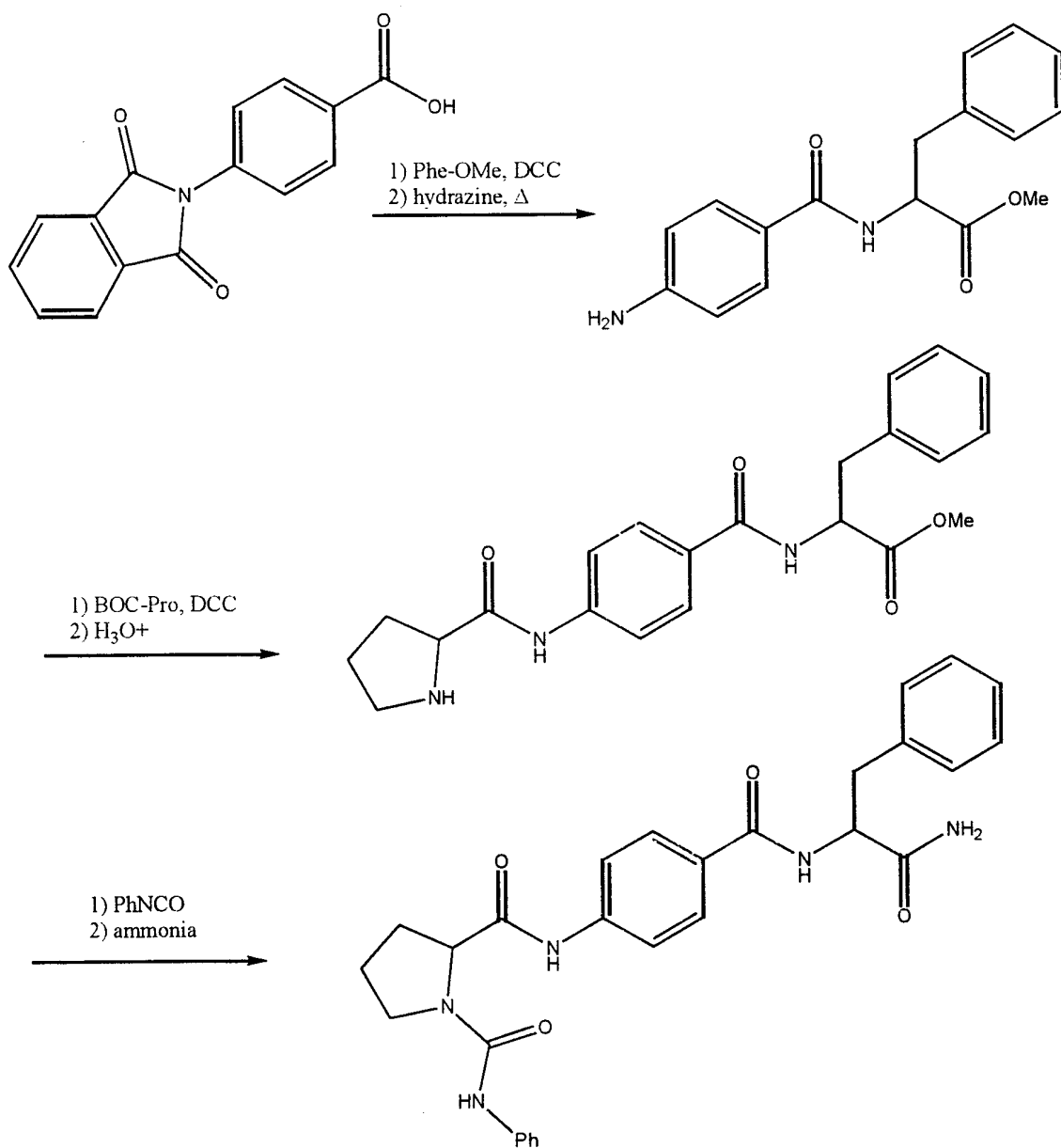
b. Synthesis of a Piperazine Acid-Containing Peptidomimetic.
