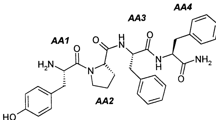
Endomorphin 2 (2) [Tyr-Pro-Phe-Phe-NH 2 ]
