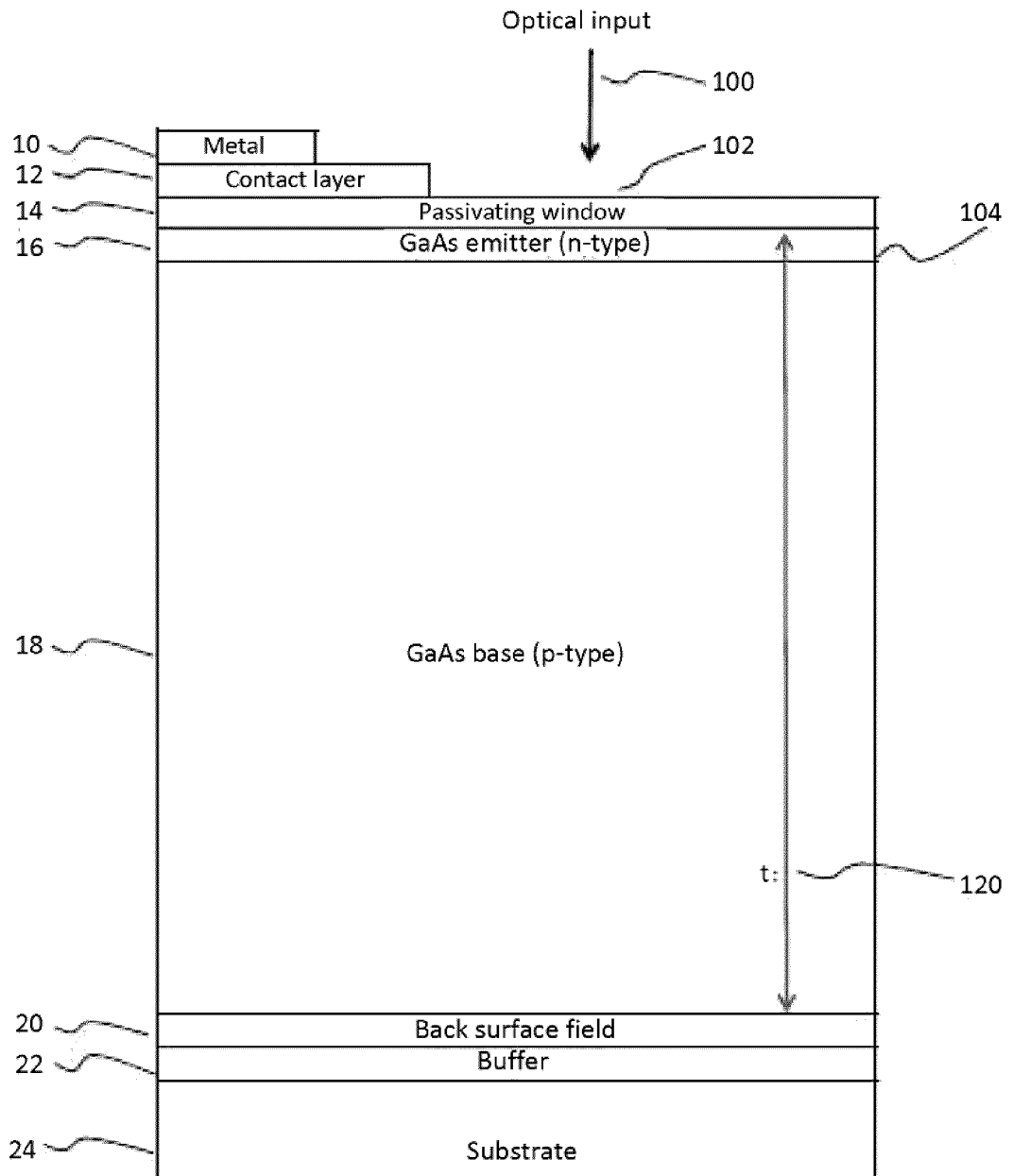
Figure 1 Prior Art
