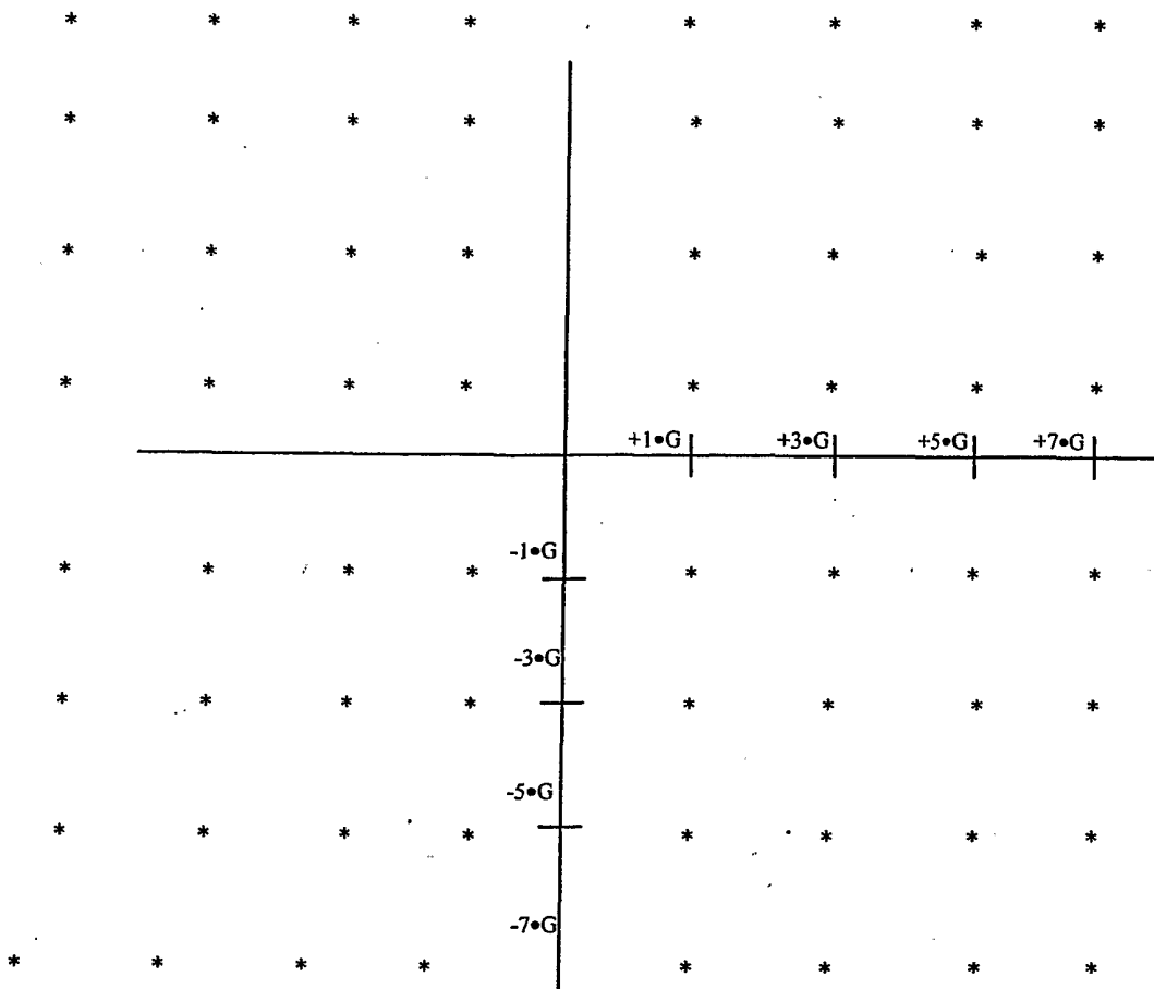
Figure 3: 64-QAM constellation
