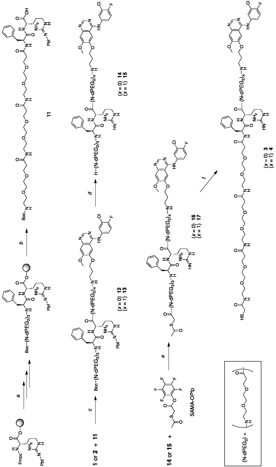
Scheme 5
