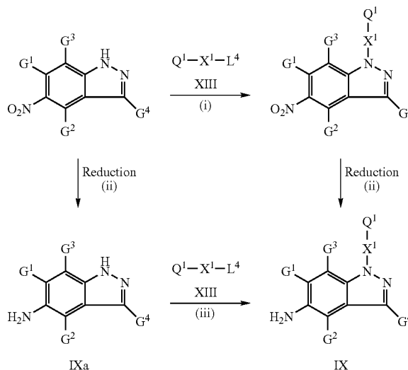
Reaction Scheme 2
