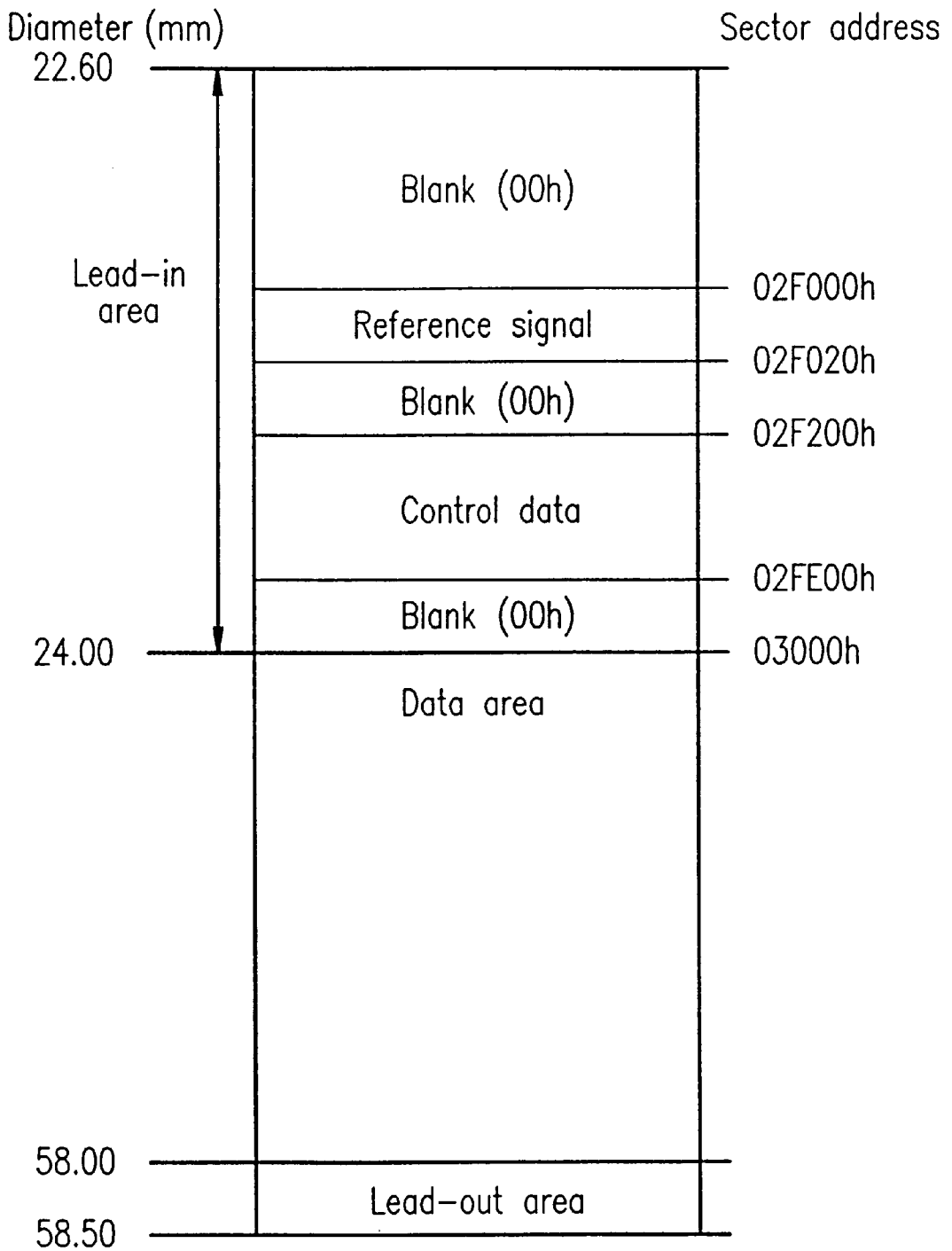
FIG. 8 PRIOR ART
