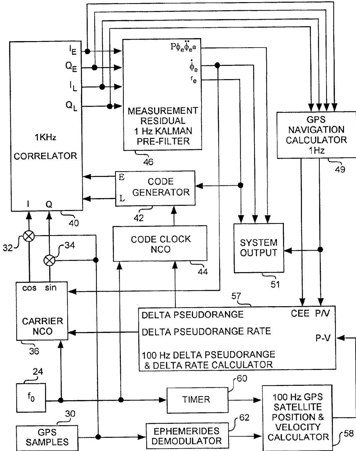
WEAK LOCK GPS NAVIGATION PROCESSOR FIG. 2A
