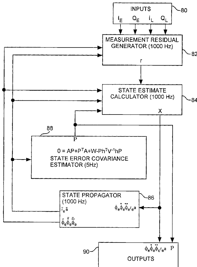
GPS SIGNAL RESIDUAL ESTIMATOR PROCESS
