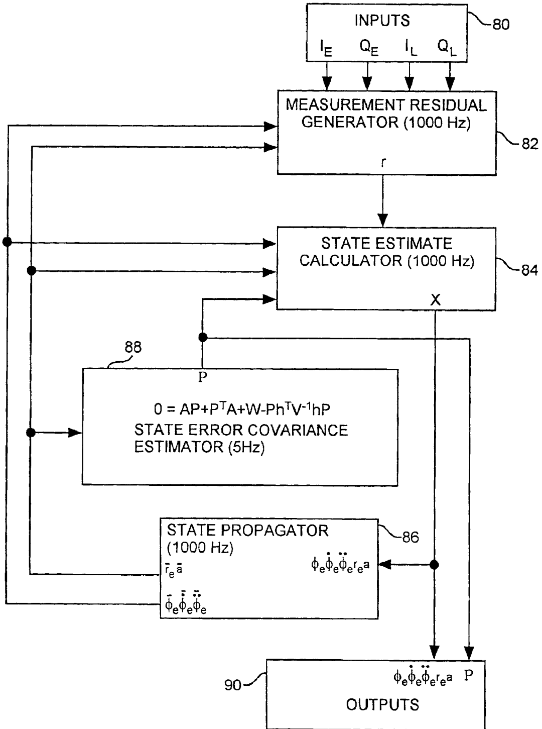
GPS SIGNAL RESIDUAL ESTIMATOR PROCESS
