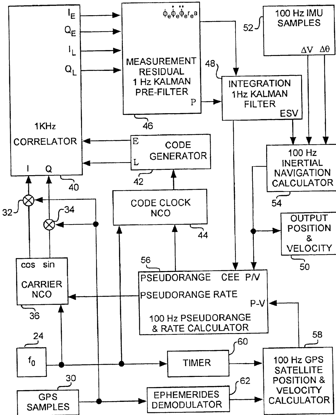
ULTRATIGHT GPS NAVIGATION PROCESSOR
