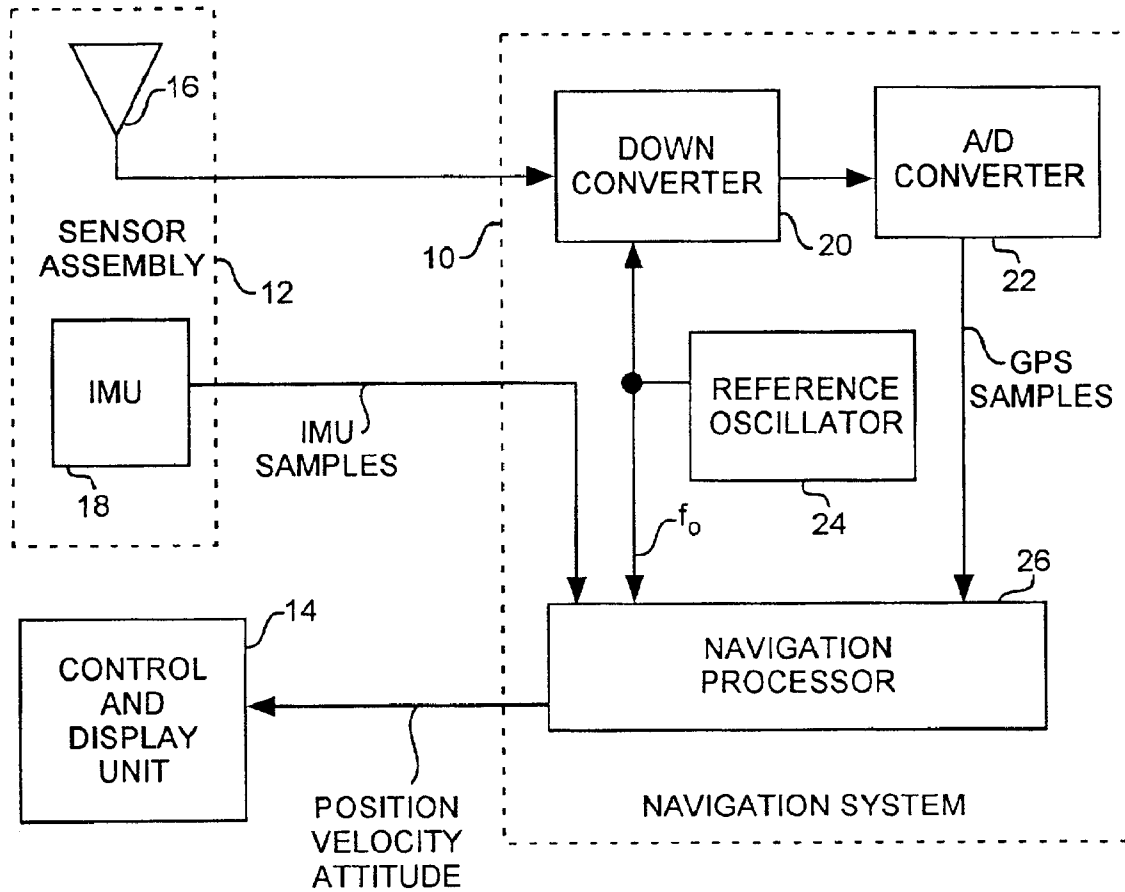
GPS INERTIAL NAVIGATION SYSTEM
