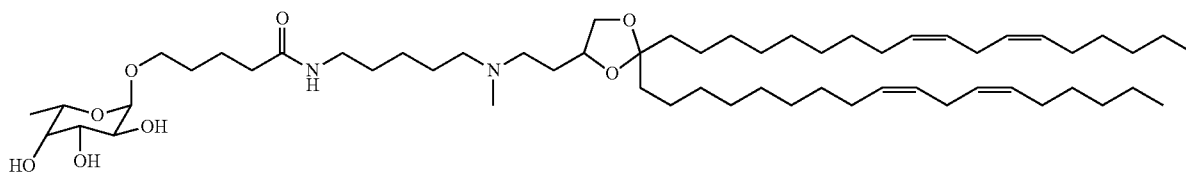
XTC 2 -Fucose
