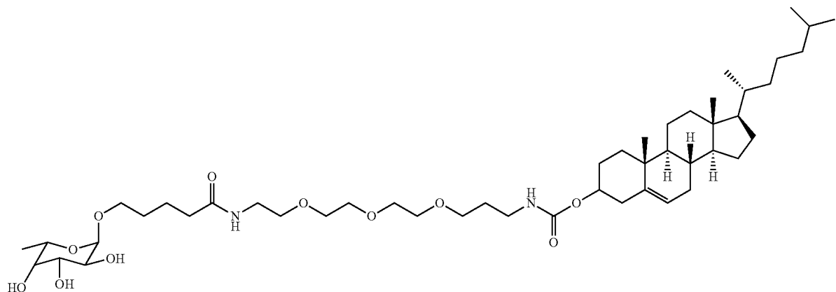
Chol-Fucose
