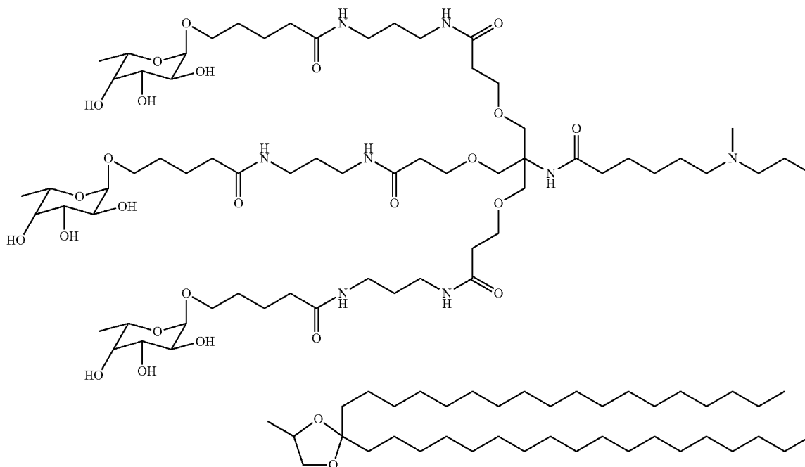
XTC 2 -Fucose 3
