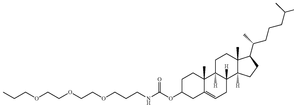
Chol-Fucose 3
