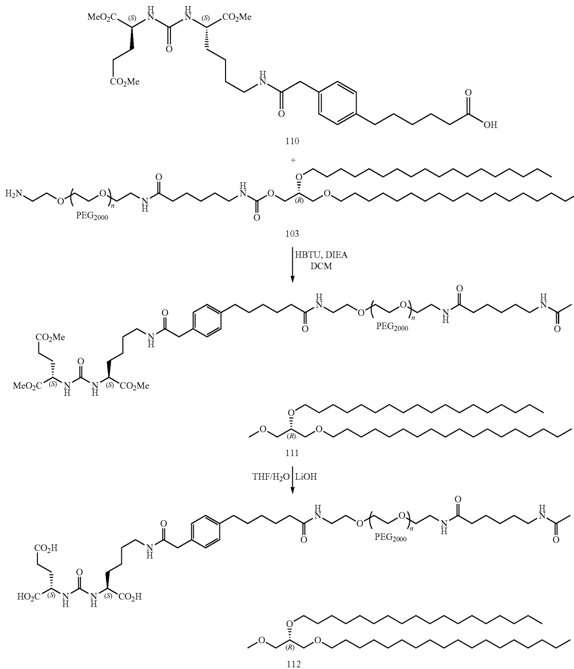
Scheme 3
