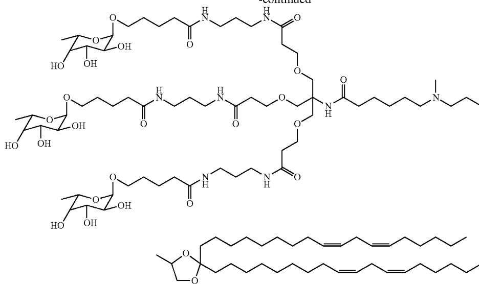
XTC 2 -Fucose 3
