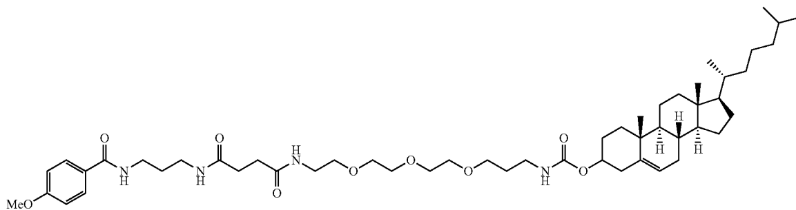
Chol-Anisamide
