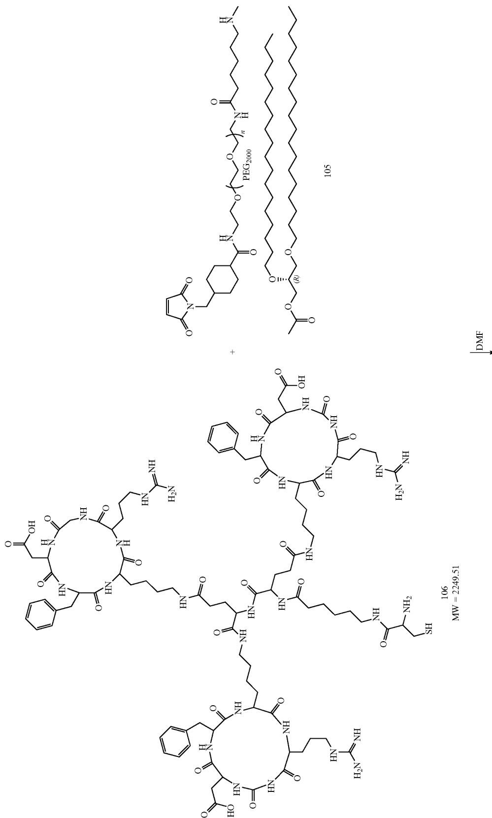
Scheme 2
