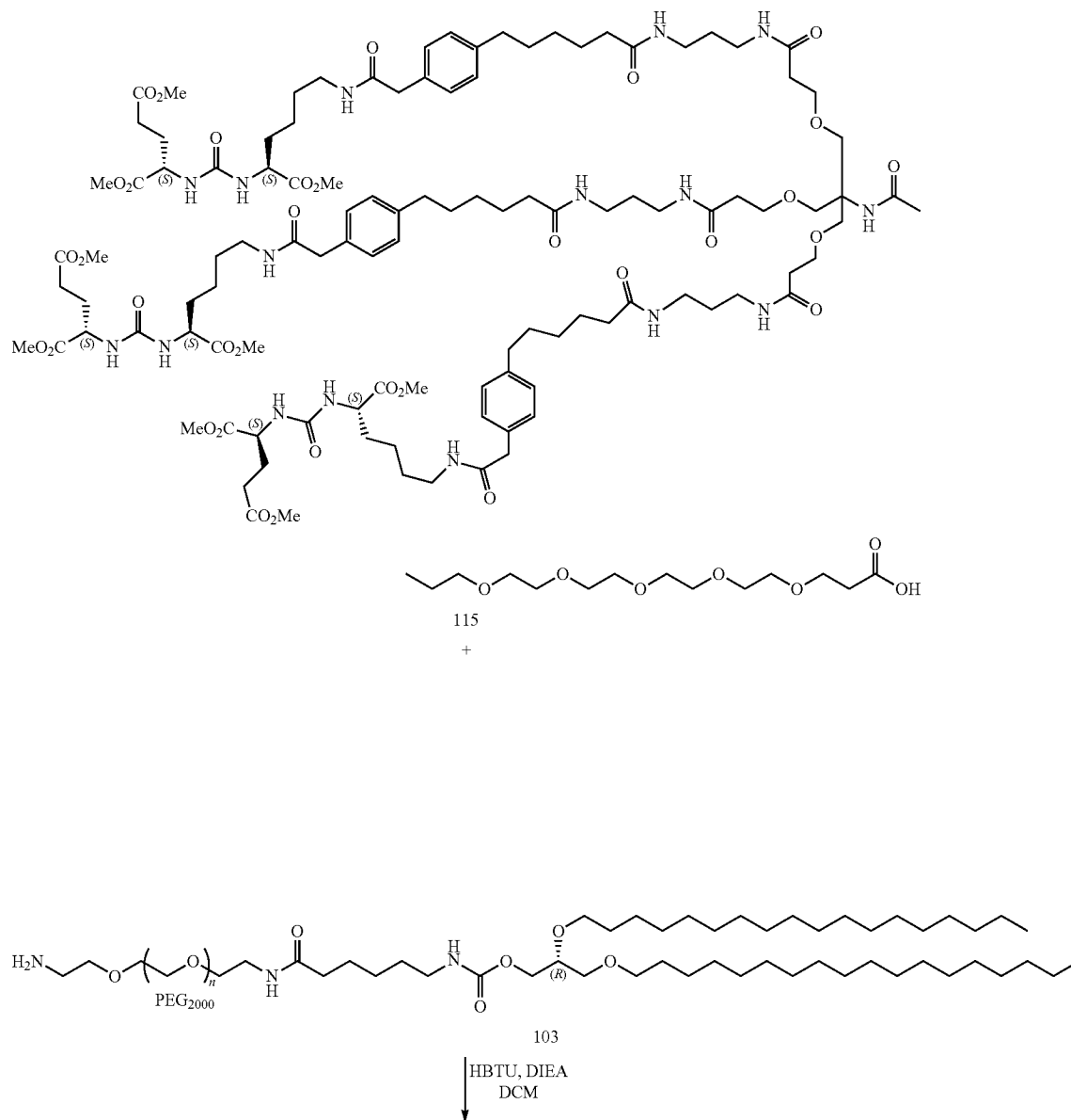
Scheme 5
