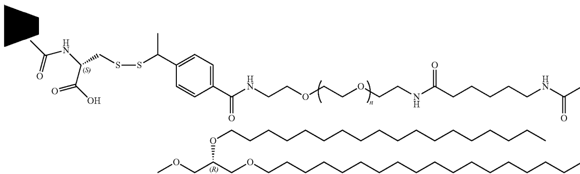
XTC 2 -Fucose 3
