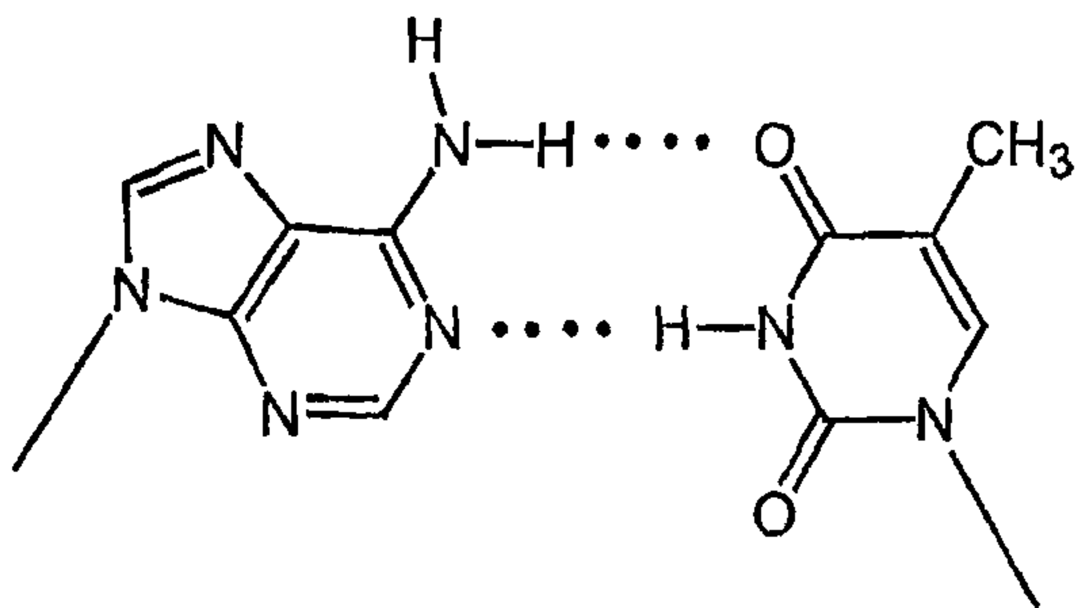
Watson Crick AT-Base Pair I antiparallel
