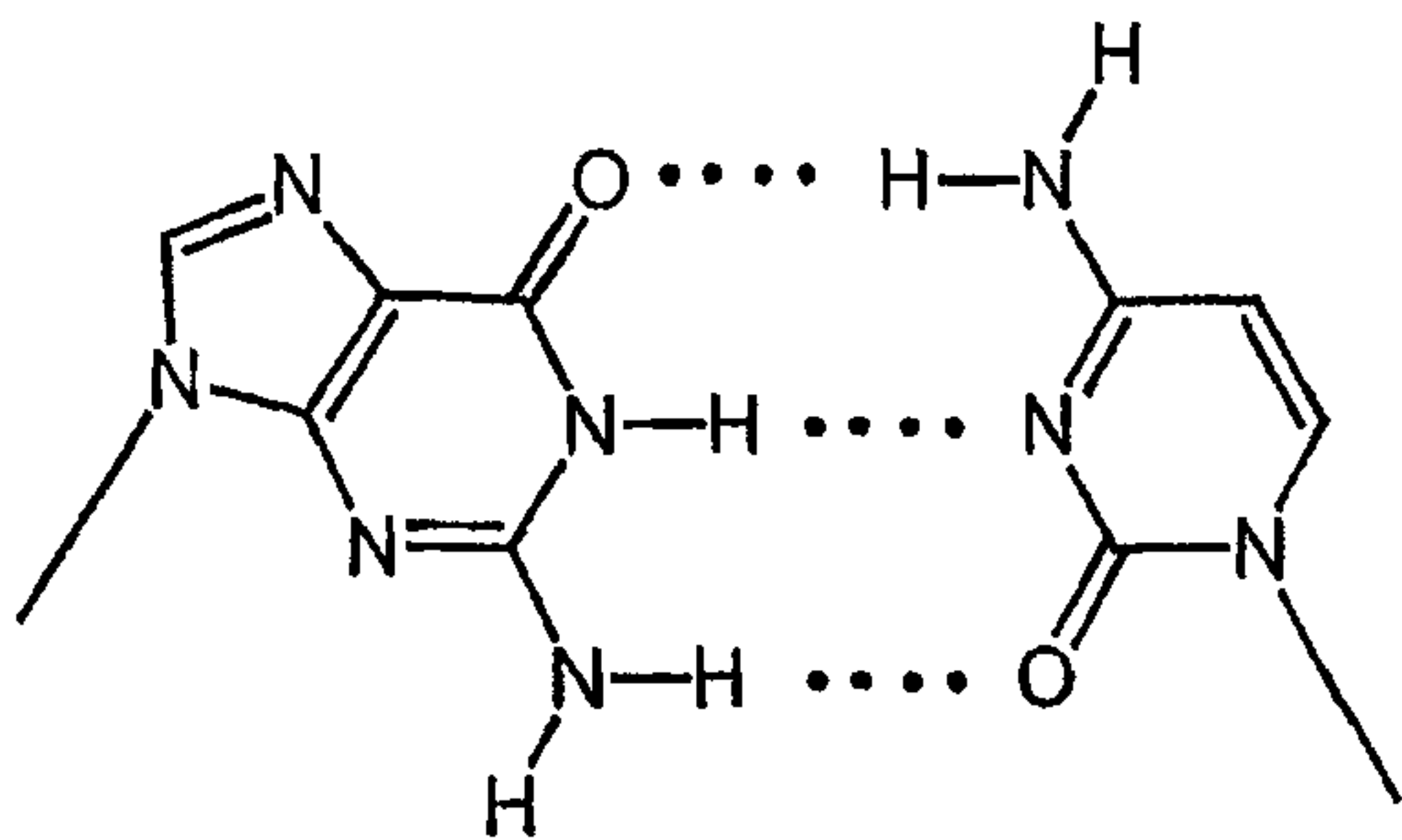
Watson Crick GC-Base Pair VII antiparallel
