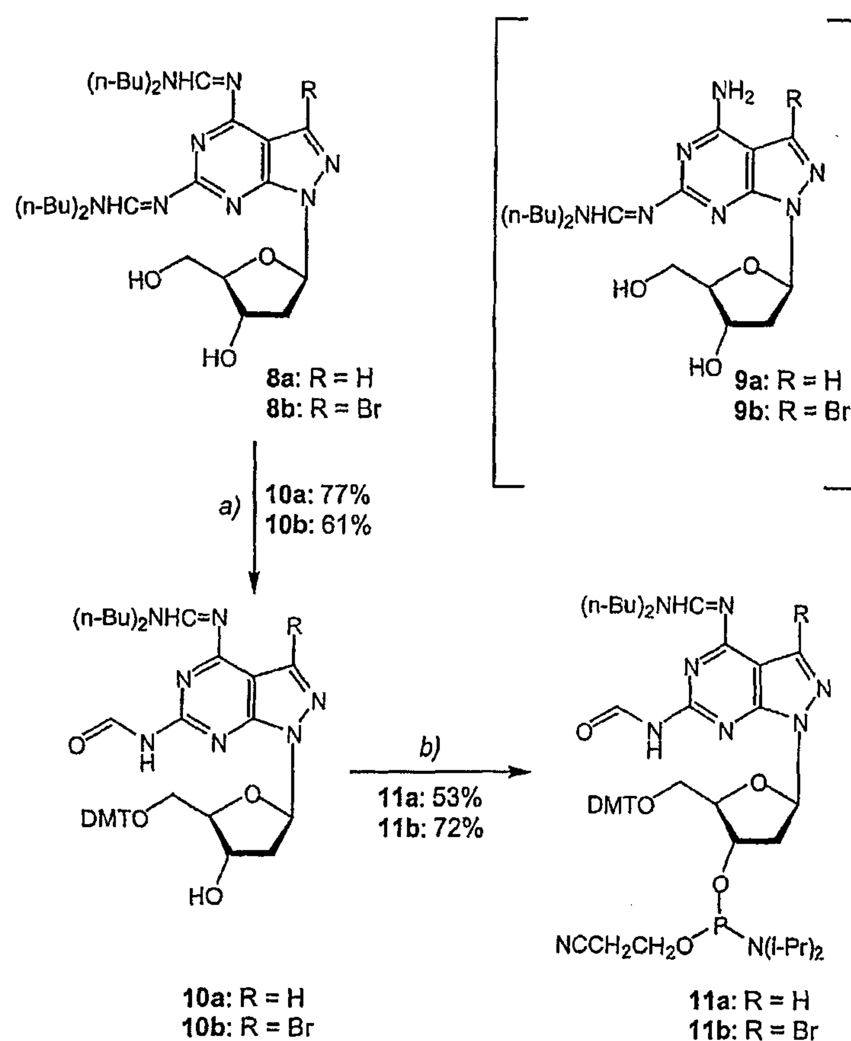
Scheme 3
