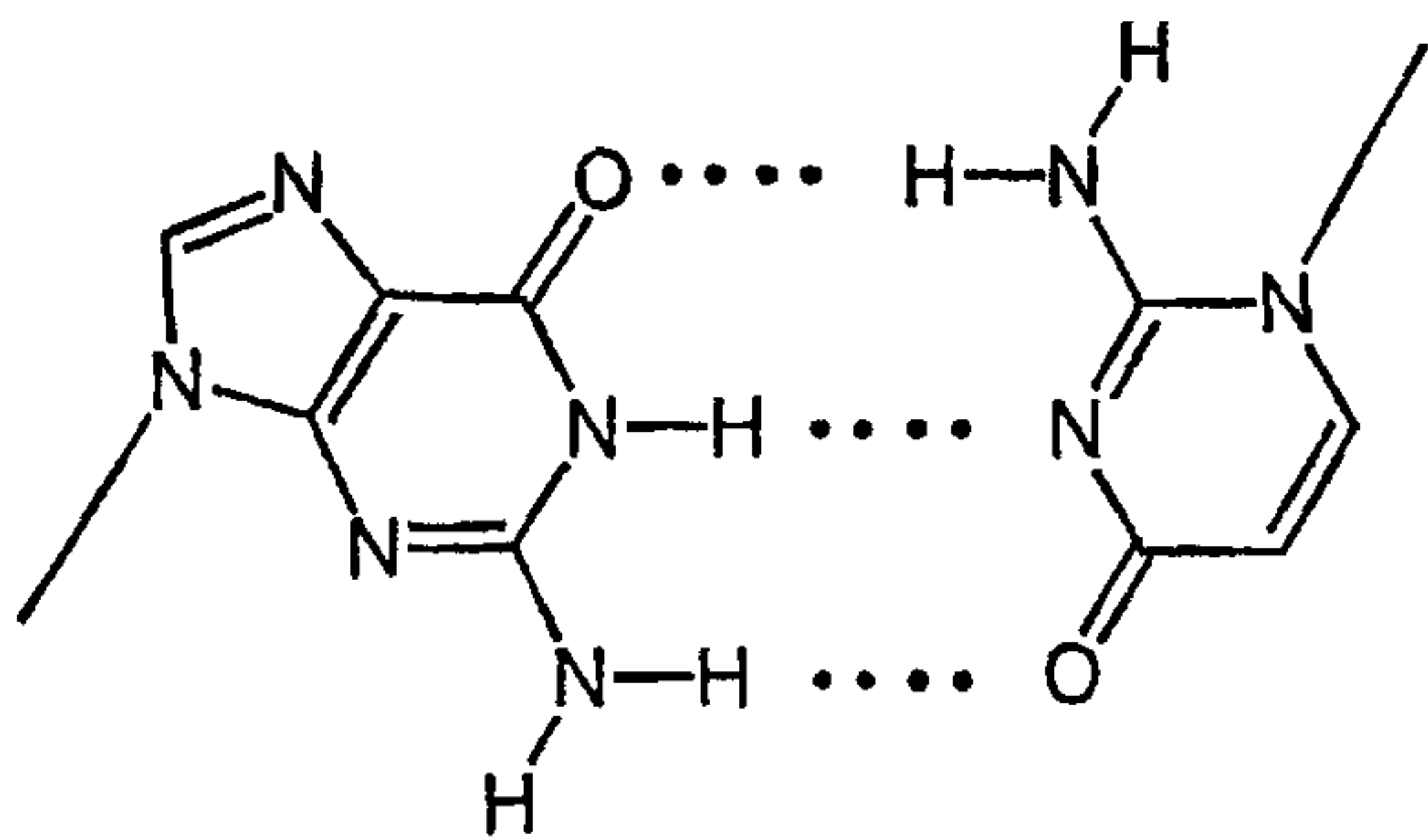
Reverse Watson Crick GiC-Base Pair IX parallel
