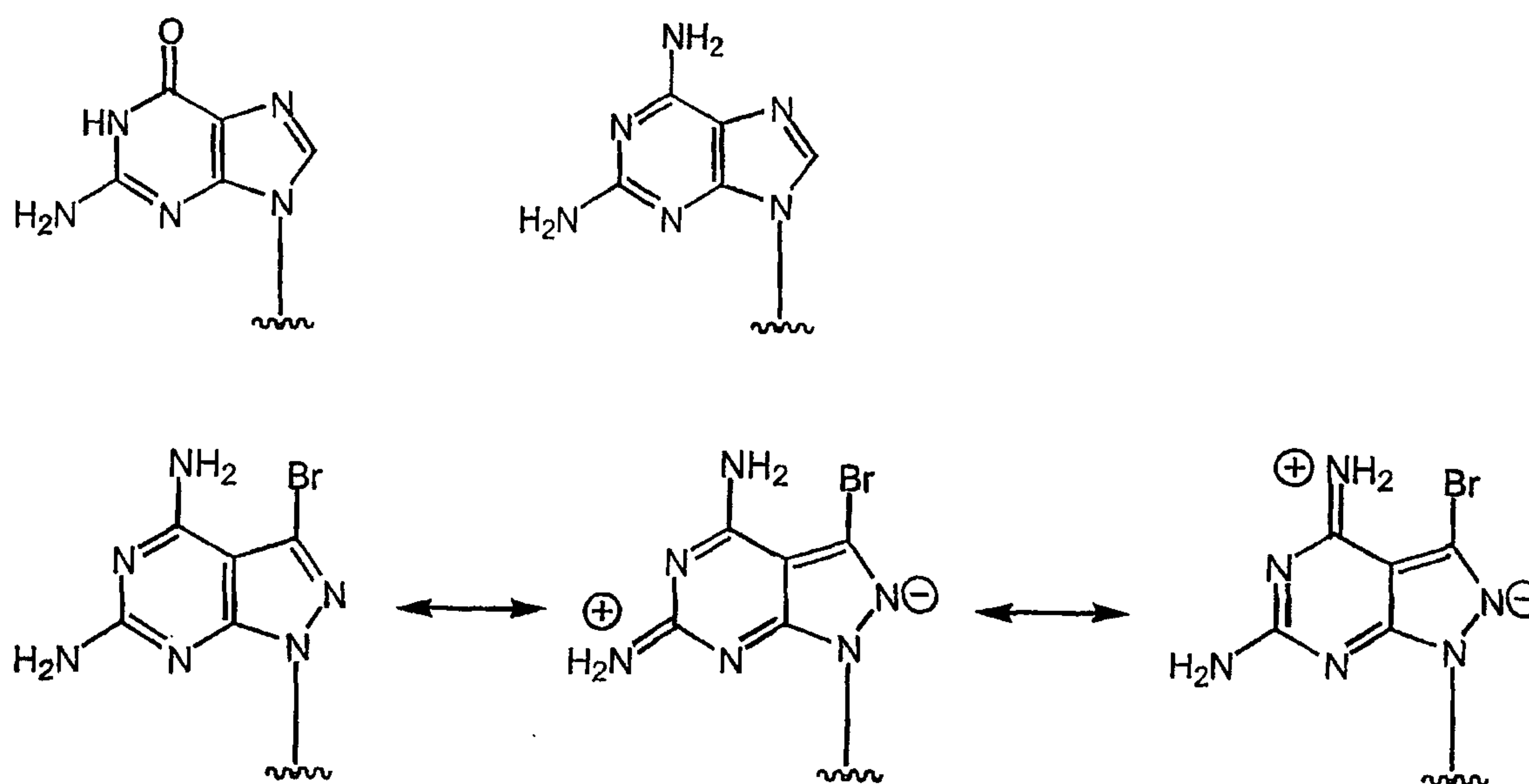
15 Scheme 5
