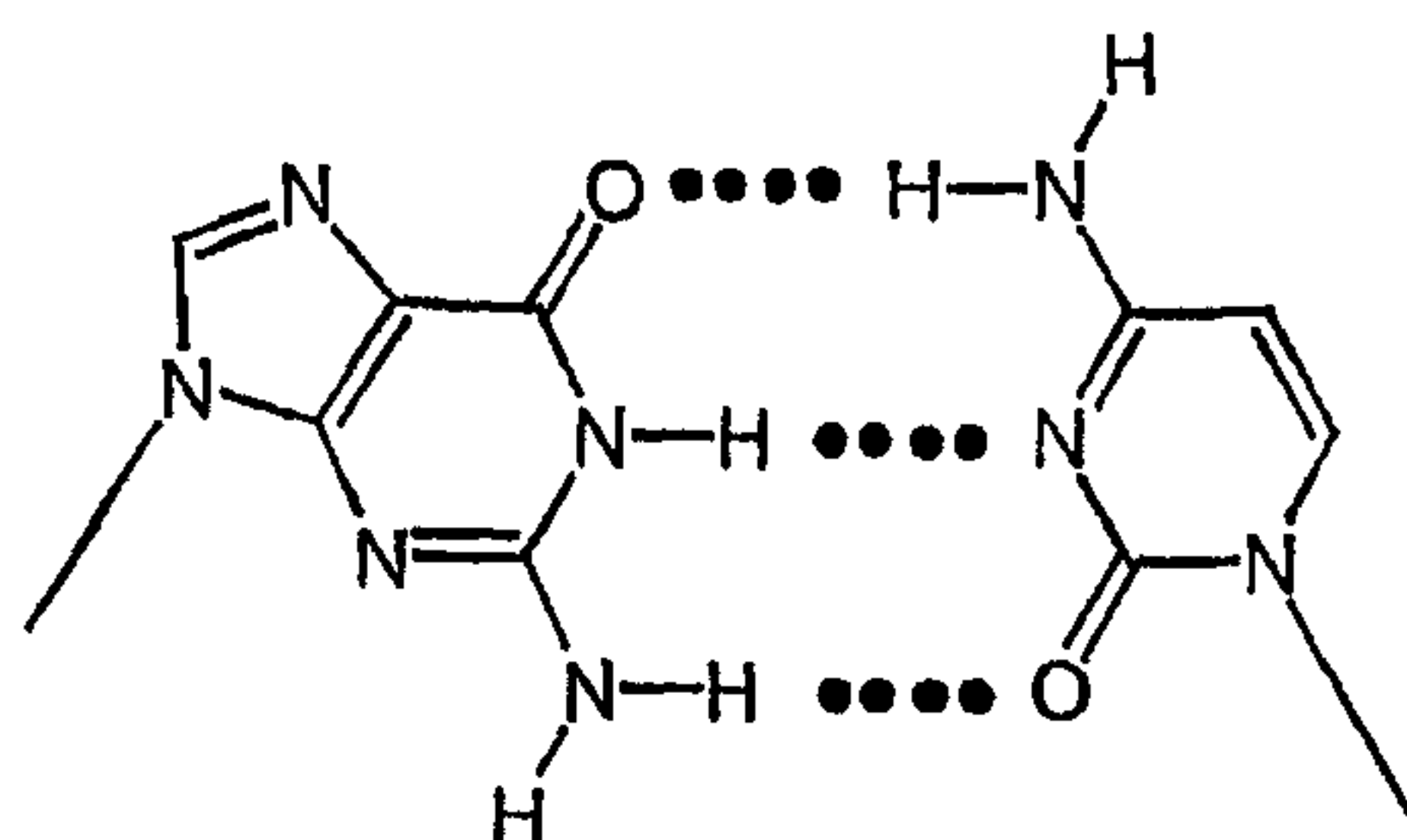
Watson Crick Base Pair III
