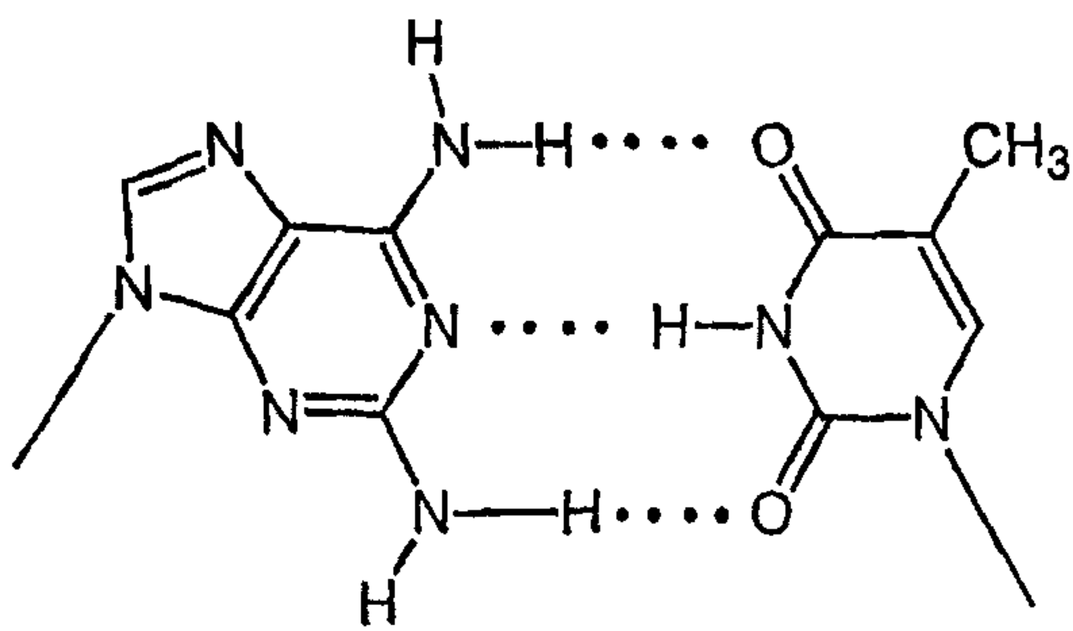
Watson Crick n^2 AT-Base Pair III antiparallel
