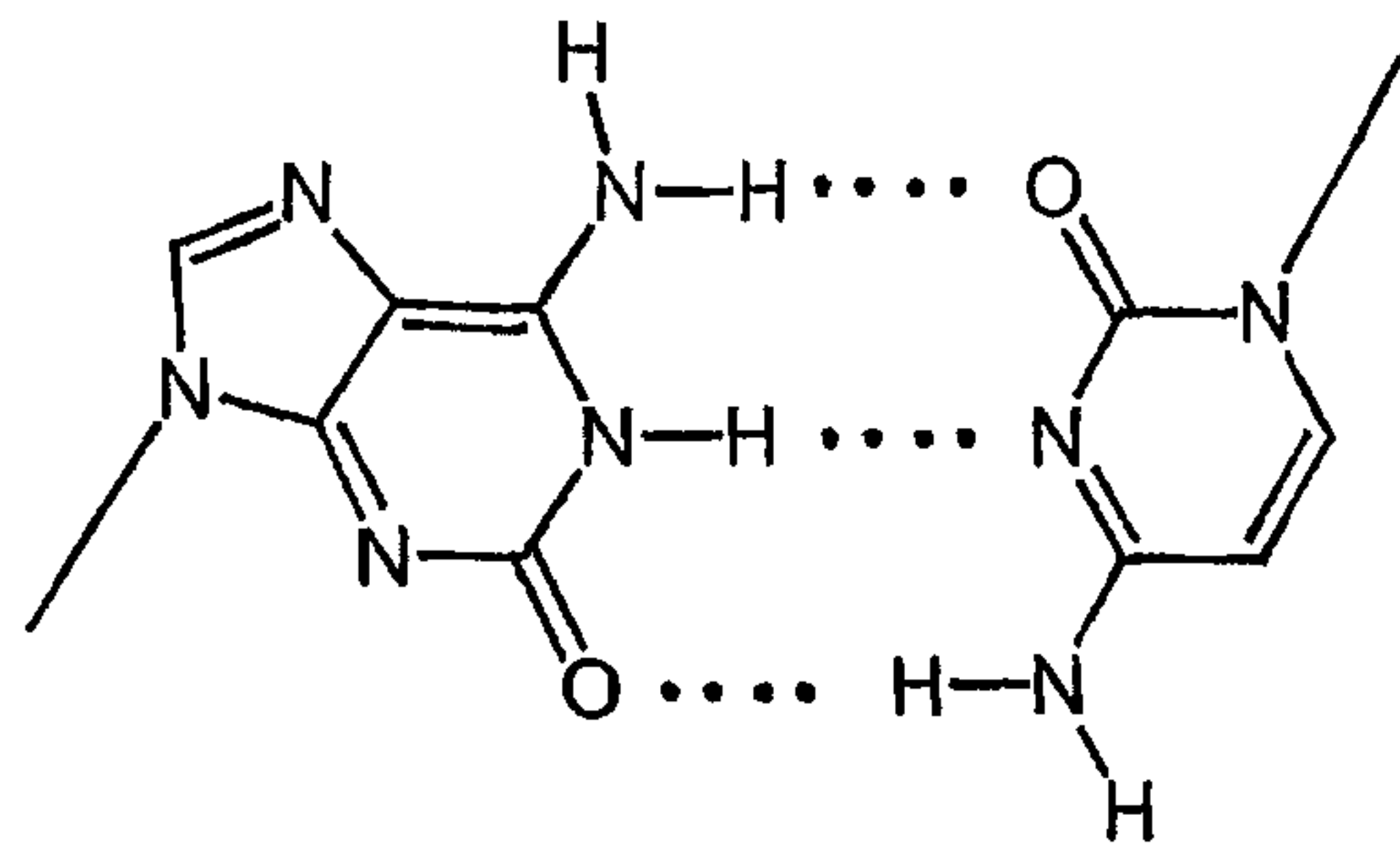
Reverse Watson Crick iGC-Base Pair VIII parallel
