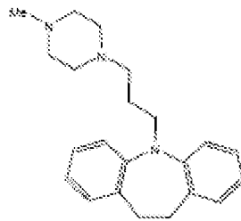
5-[3-(4-Methyl-piperazine-1-yl)-propyl]-10,11-dihydro-5H-dibenzo[b,f]azepine
