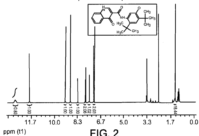
1 H NMR Spectrum of Compound 1
