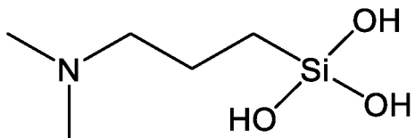
- (2-Dimethylaminoethyl)triethoxysilan.
