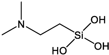
1-(2-Dimethylaminoethyl)silanetriol
