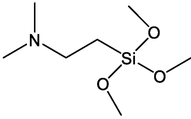
1-(2-Dimethylaminoethyl)silanetriol
