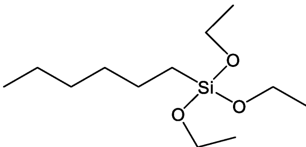
- n-Hexyltriethoxysilan
