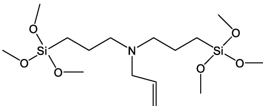
- N,N-Bis[3-(trimethoxysilyl)propyl]-2-propen-1-amin
