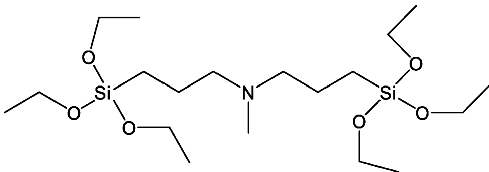
- N-Methyl-3-(trimethoxysilyl)-N-[3-(trimethoxysilyl)propyl]-1-propanamin
