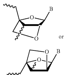
Scheme 5
