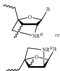
Scheme 4
