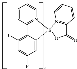
Irpic
