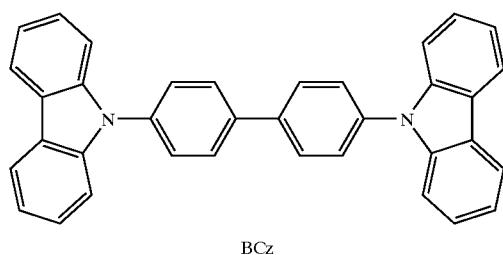
BCz
