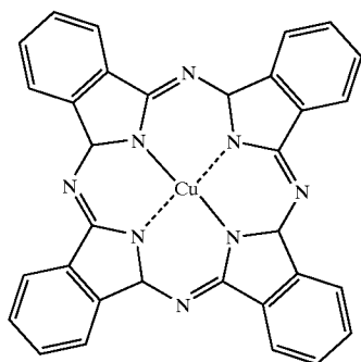
CuPc
