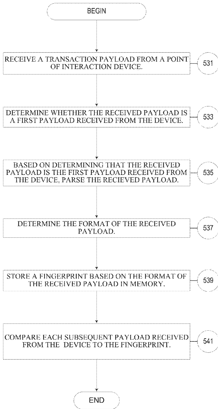
FIG. 5B EXEMPLARY FINGERPRINT PROCESS
