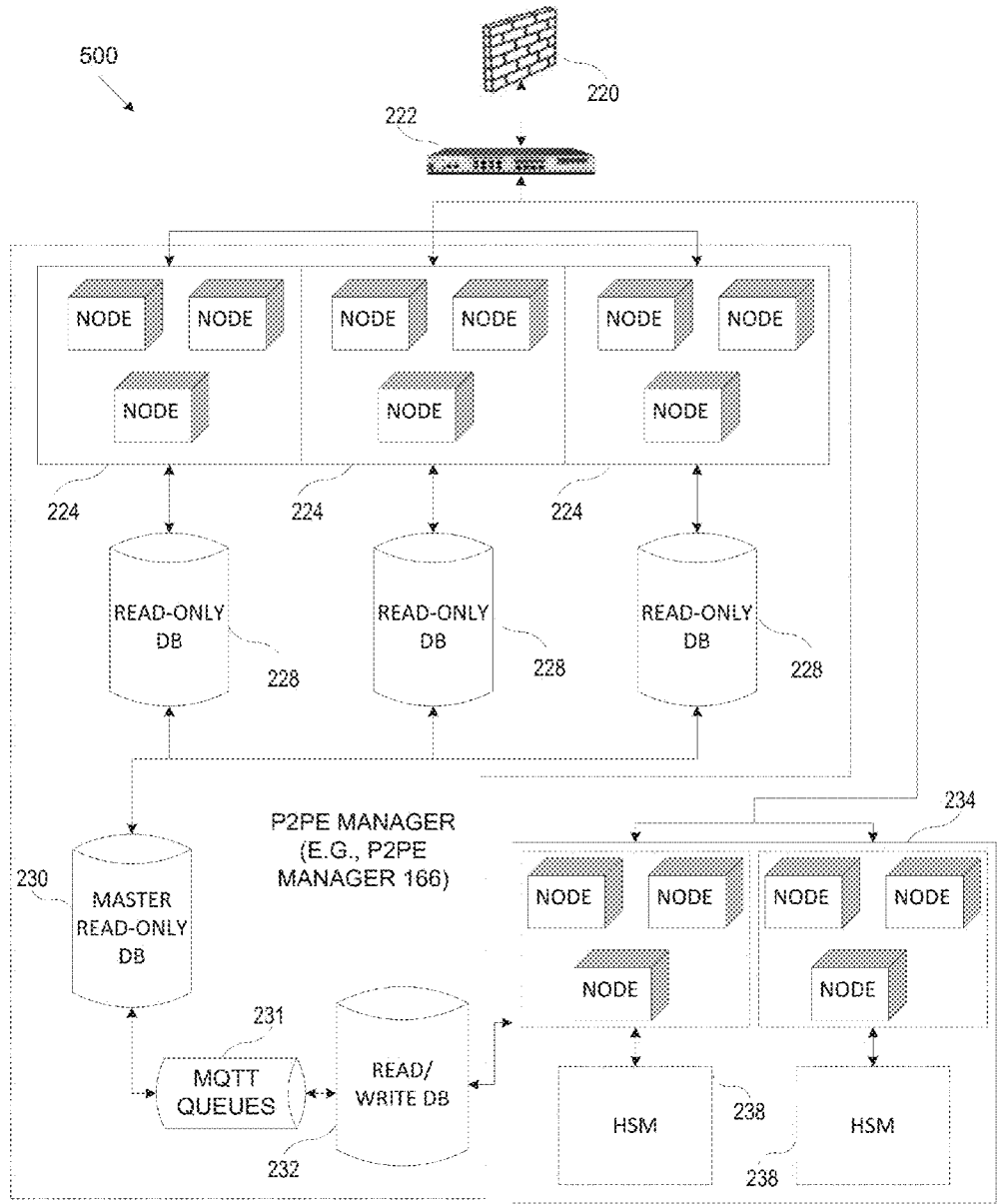
FIG. 2C ALTERNATIVE EXEMPLARY P2PE MANAGER SYSTEM ARCHITECTURE
