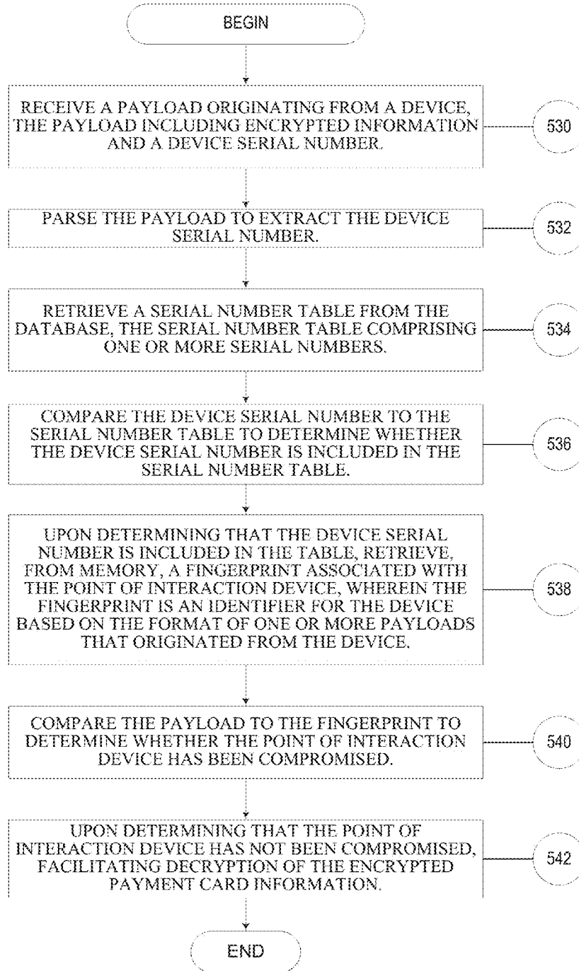
FIG. 5A EXEMPLARY DECRYPTION PROCESS
