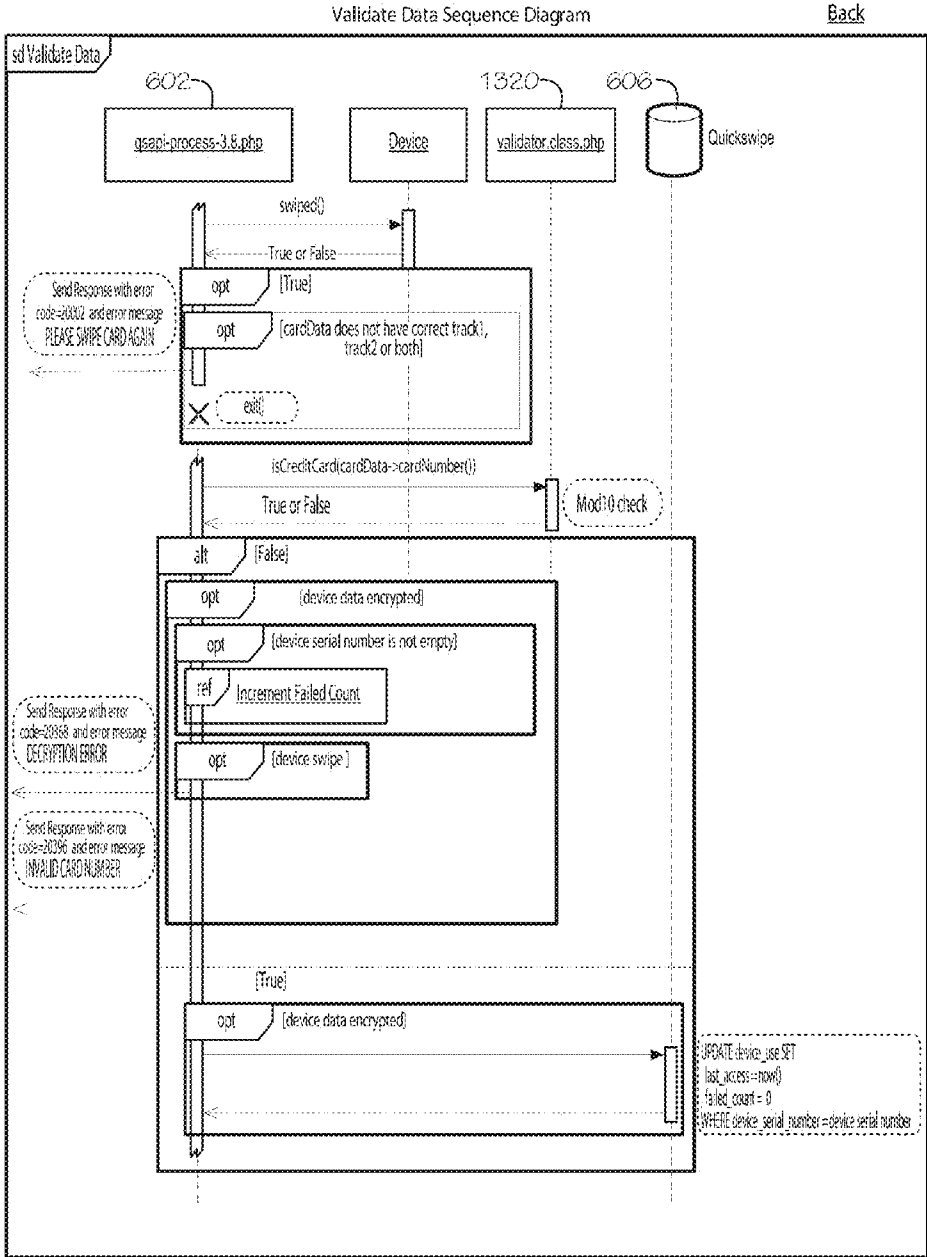
UML OF EXEMPLARY VALIDATION SEQUENCE FIG. 13
