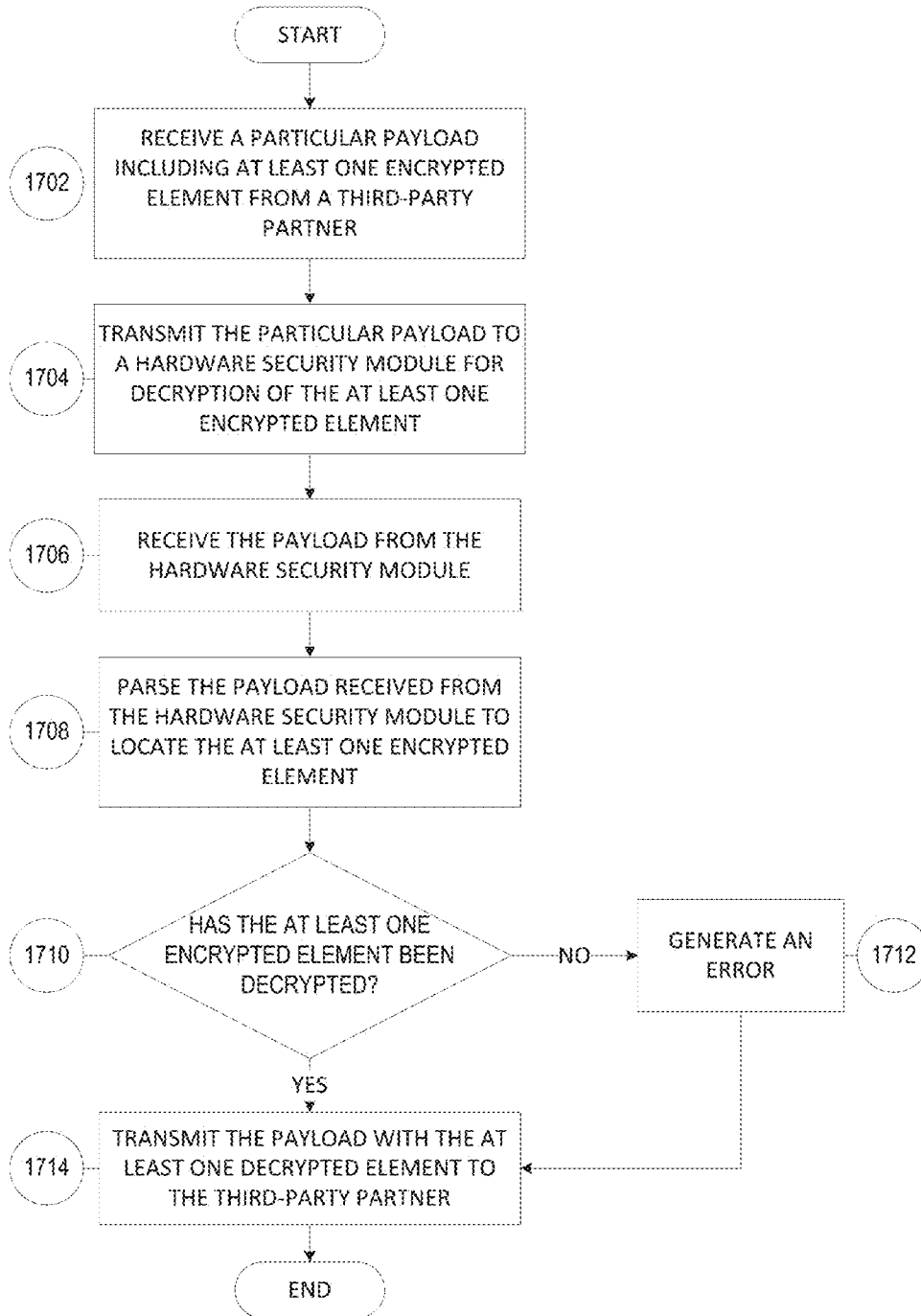
FIG. 17 EXEMPLARY DECRYPTION VERIFICATION PROCESS
