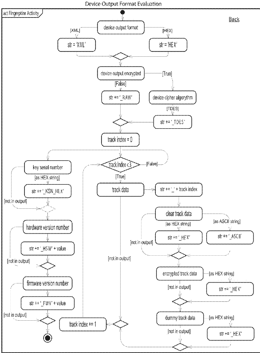
UML OF EXEMPLARY OUTPUT EVALUATION
