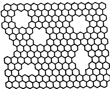
OXYGEN PLASMA
