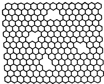
ARGON PLASMA
