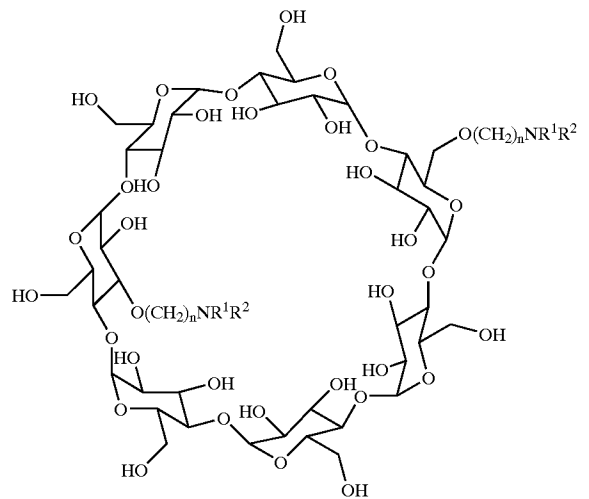
Tertiary Amino Beta Cyclodextrin; or
