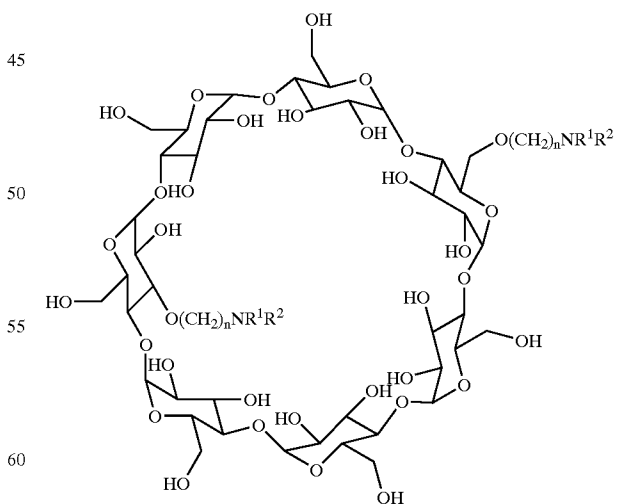
gamma-Cyclodextrin: 8 D-glucose rings containing 24 hydroxyl groups.
