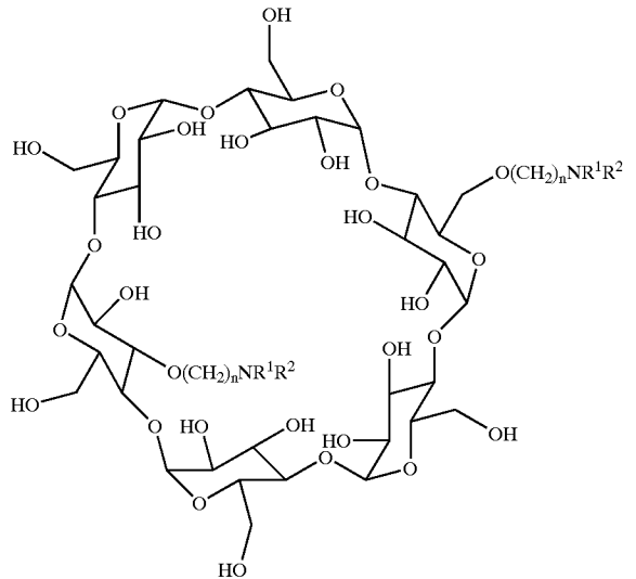
beta-Cyclodextrin: 7 D-glucose rings containing 21 hydroxyl groups; or
