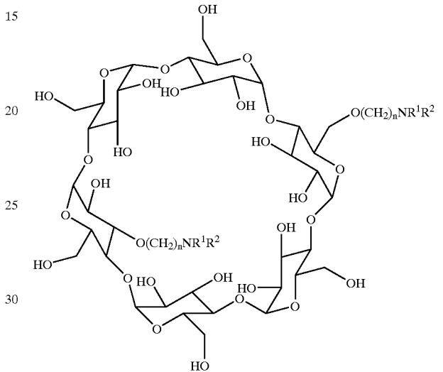
beta-Cyclodextrin: 7 D-glucose rings containing 21 hydroxyl groups; or
