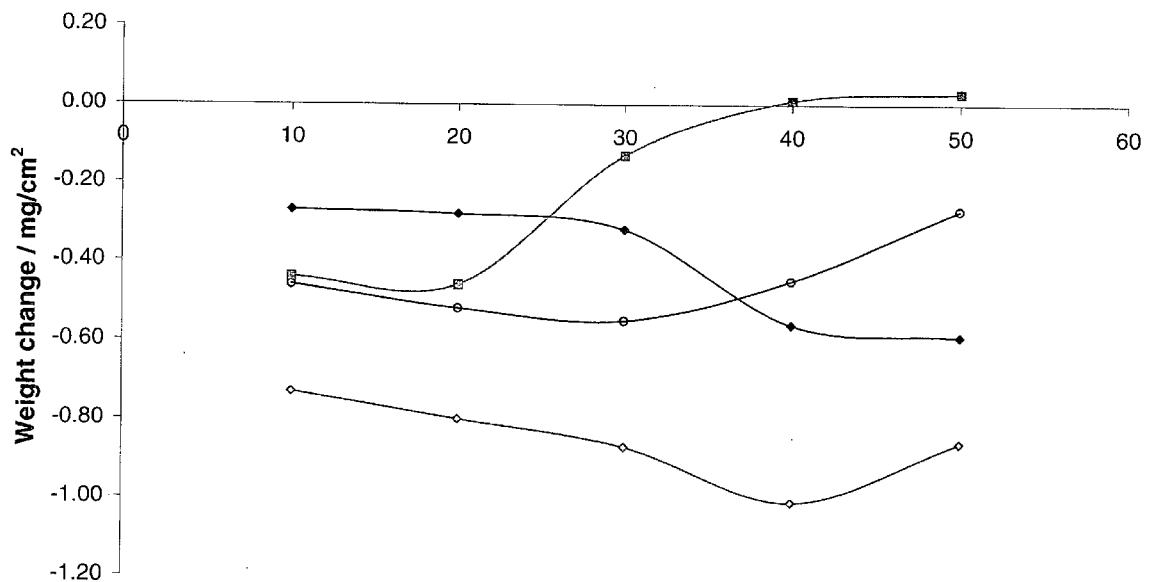
Concentration of solvent component / % of Vol. ◆ N-methyl-2-pyrrolidone ○ Gamma-butyrolactone ■ Equal concentrations of N-methyl-2-pyrrolidone and Gamma-butyrolactone actual results ◇ Equal concentrations of N-methyl-2-pyrrolidone and Gamma-butyrolactone expected results
