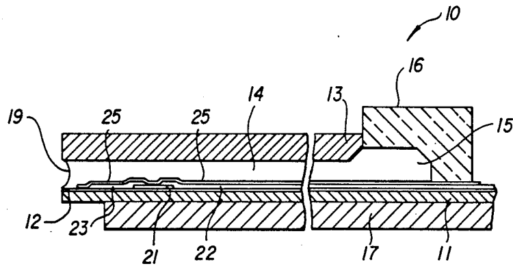
FIG. 1 (PRIOR ART)
