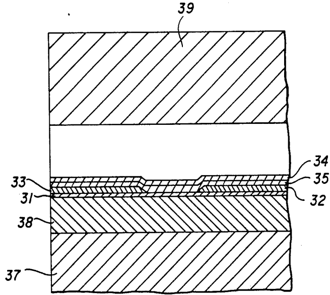
FIG. 3 (PRIOR ART)
