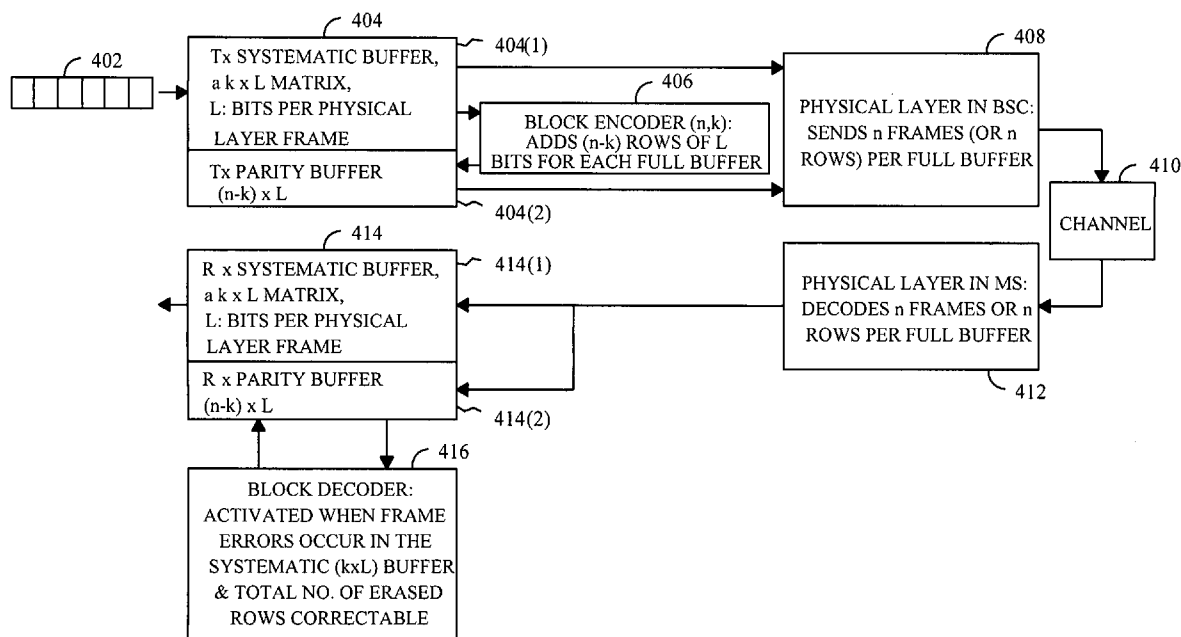
REED-SOLOMAN OUTER CODE BLOCK DIAGRAM
