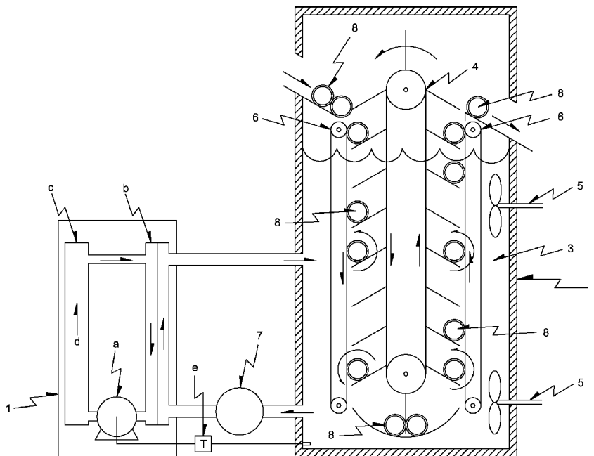
EQUIPMENT FOR FAST CHILLING OF CONTAINERIZED BEVERAGES
