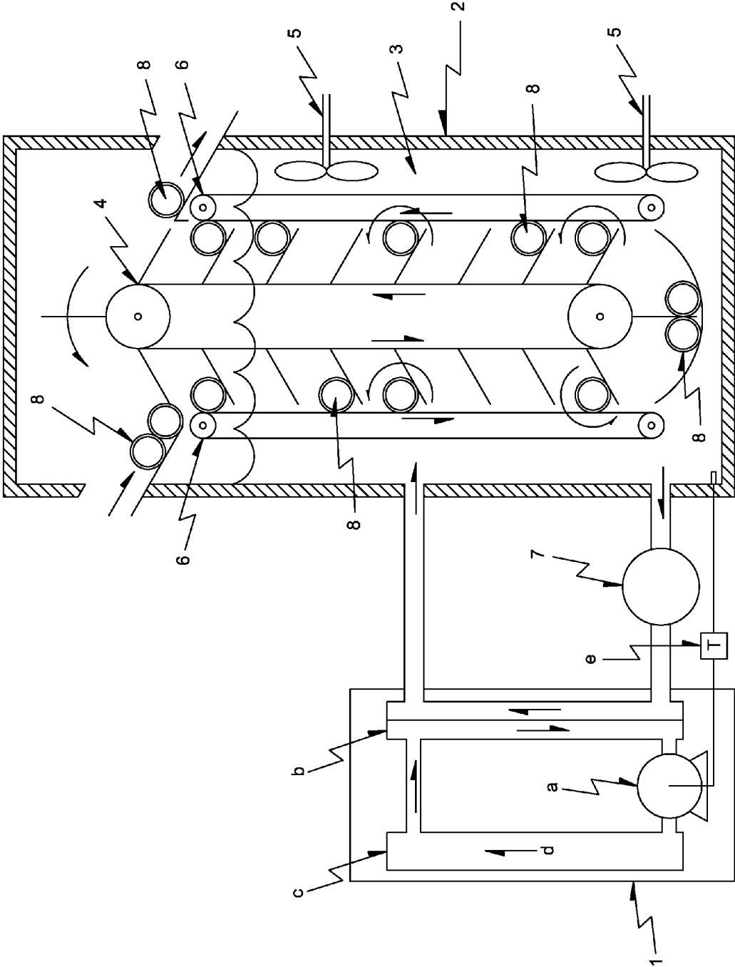
EQUIPMENT FOR FAST CHILLING OF CONTAINERIZED BEVERAGES
