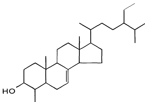
Formula (8): 4-methylstigmast-7-en-3-ol
