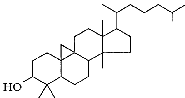
Formula (2): 9,19-cyclolanostan-3-ol
