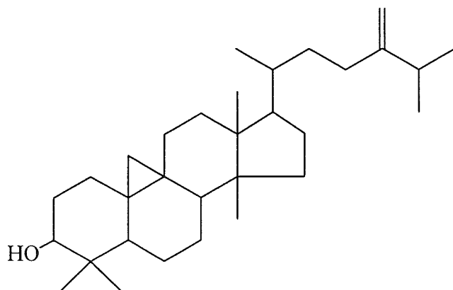
Formula (3): 24-methylene-9,19-cyclolanostan-3-ol
