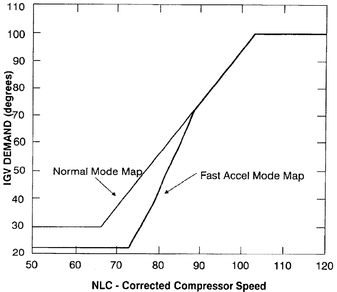
Steady-State IGV Schedules
