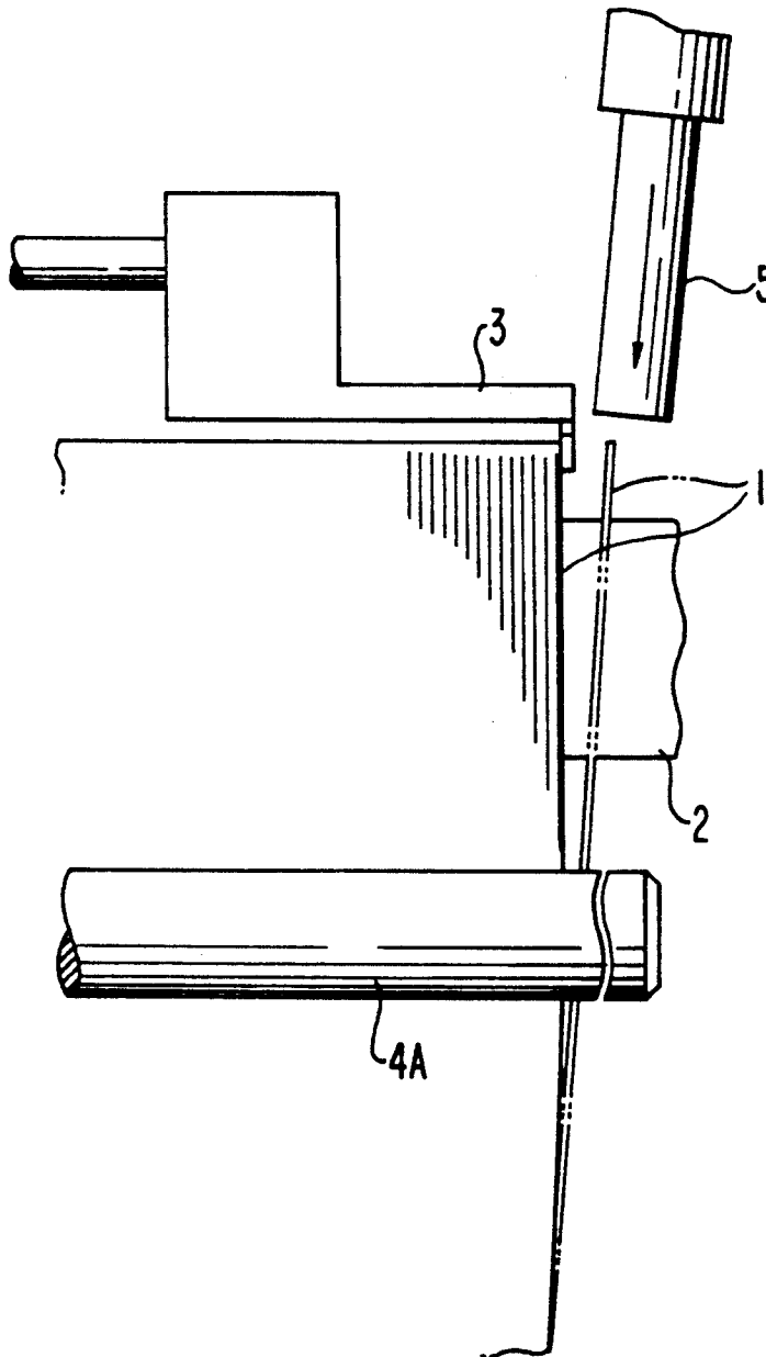
FIG. 16 (PRIOR ART)
