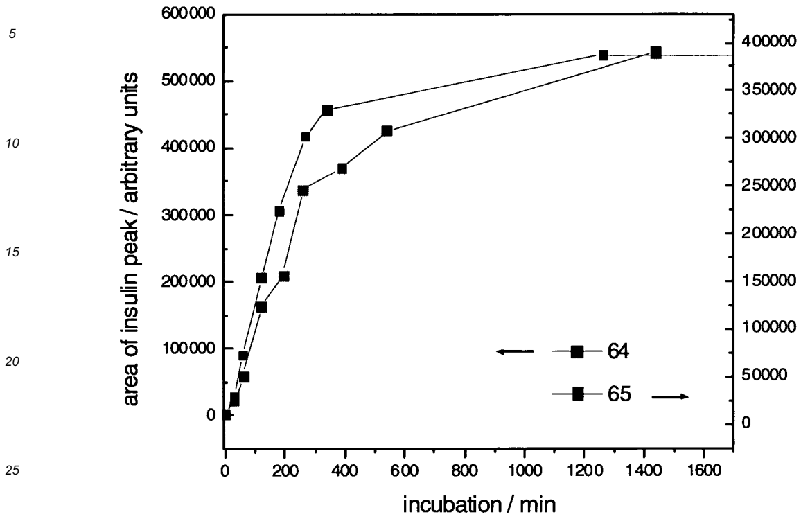
Fig. 4 : In vitro release of insulin from Insulin MPIC 64 or 65 , respectively. Kinetics were determined by HPLC using UV detection at 215 nm.
