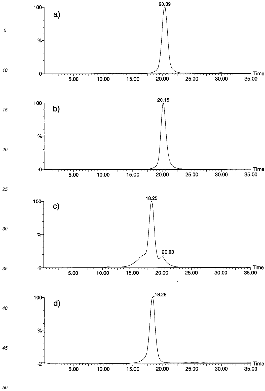
Fig. 1 : Size exclusion chromatograms of a) native Hb, b) 39 , c) reaction mixture 40 , and d) purified covalent Hemoglobin MPIC 40 . UV signals were recorded at 280 nm.
