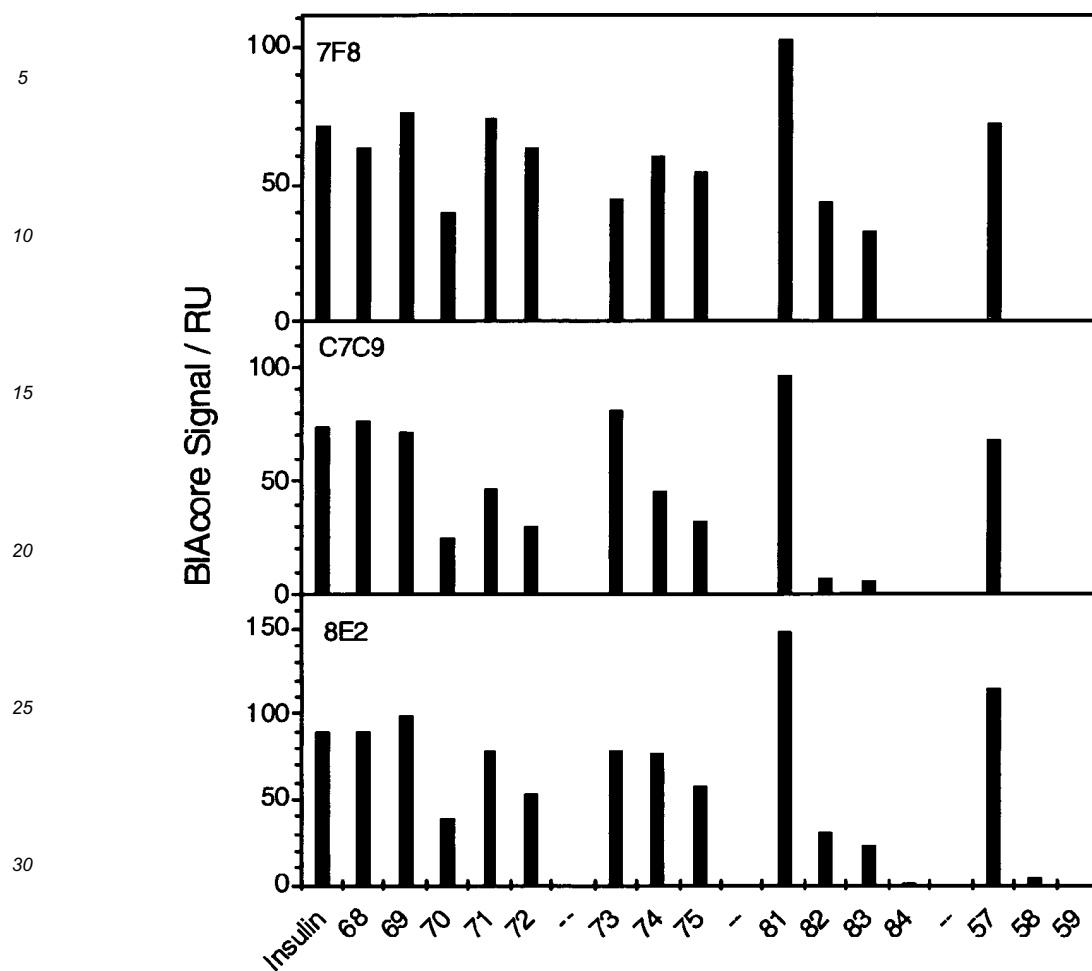
Fig. 6 : Binding of insulin or insulin conjugates to immobilized murine anti insulin antibodies (clones 8E2, C7C9 and 7F8).
