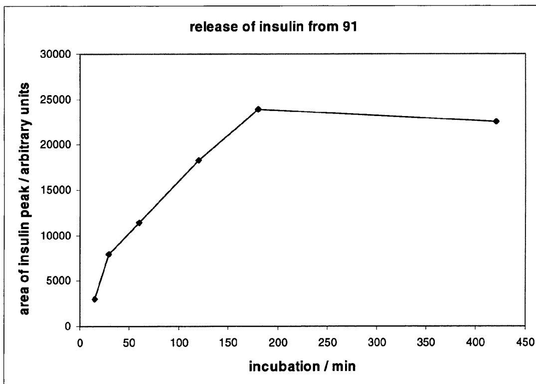
Fig. 5: Release of insulin from dendrimer prodrugs 90 (top) and 91 (below). Free insulin was quantified by HPLC using UV detection at 215 nm.
