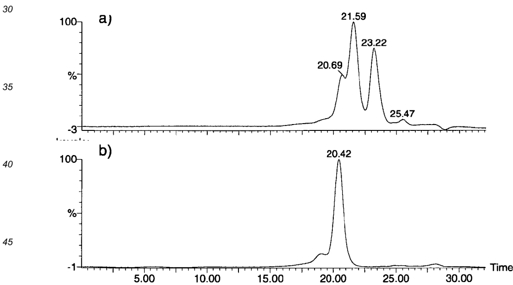
50 Fig. 3 : Size exclusion chromatograms of a) reaction mixture resulting from linker cleavage procedure performed on 50a , b) Insulin MPIC 50a . UV signals were recorded at 280 nm.
