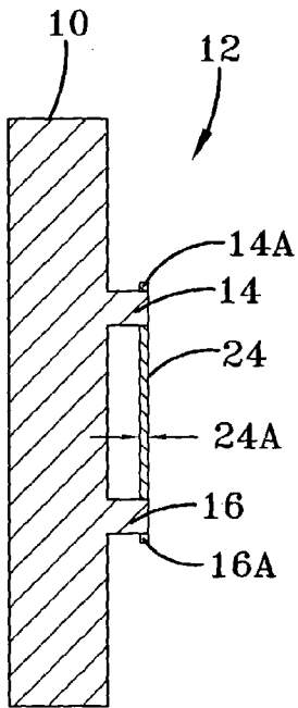
FIG-3B PRIOR ART
