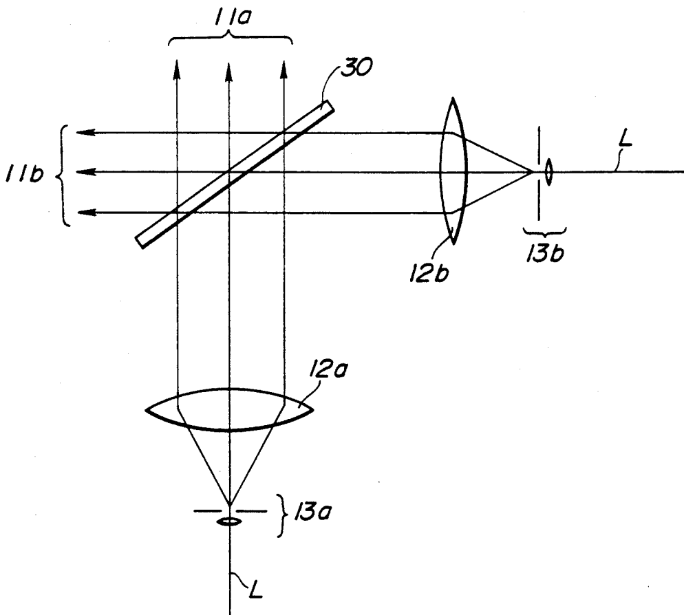
FIG. 9 (PRIOR ART)
