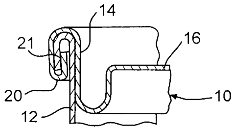
FIG. 2 PRIOR ART
