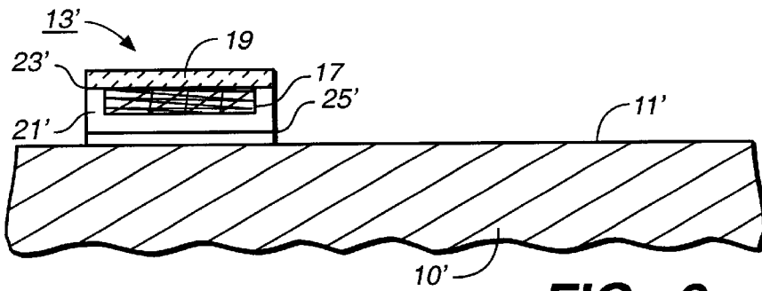
FIG. 2 (Section I-I)
