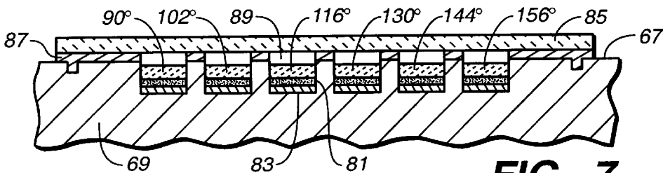
FIG. 7 (Section II-II)
