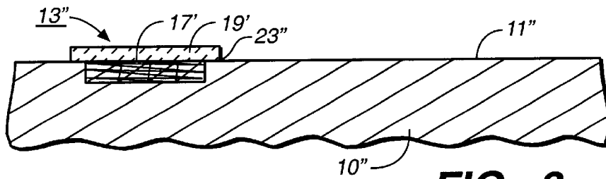
FIG. 3 (Section I-I)
