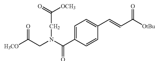
3-[4-(Bis-methoxycarbonylmethyl-carbamoyl)-phenyl]-acrylic acid tert-butyl ester (2)
