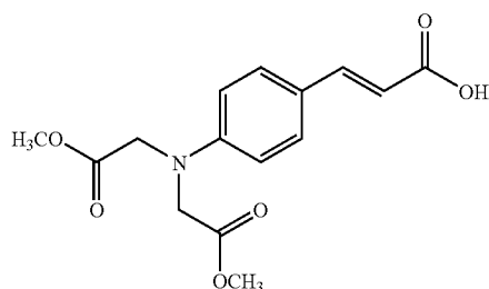
3-[4-(Bis-methoxycarbonylmethyl-amino)-phenyl]-acrylic acid (8)
