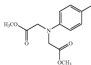
[(4-Iodo-phenyl)-methoxycarbonylmethyl-amino]-acetic acid methyl ester (7)
