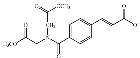
3-[4-(Bis-methoxycarbonylmethyl-carbamoyl)-phenyl]-acrylic acid (3)
