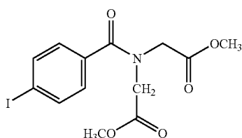
[(4-Iodo-benzoyl)-methoxycarbonylmethyl-amino]-acetic acid methyl ester (1)
