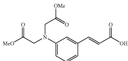
3-[3-(Bis-methoxycarbonylmethyl-amino)-phenyl]-acrylic acid (6)
