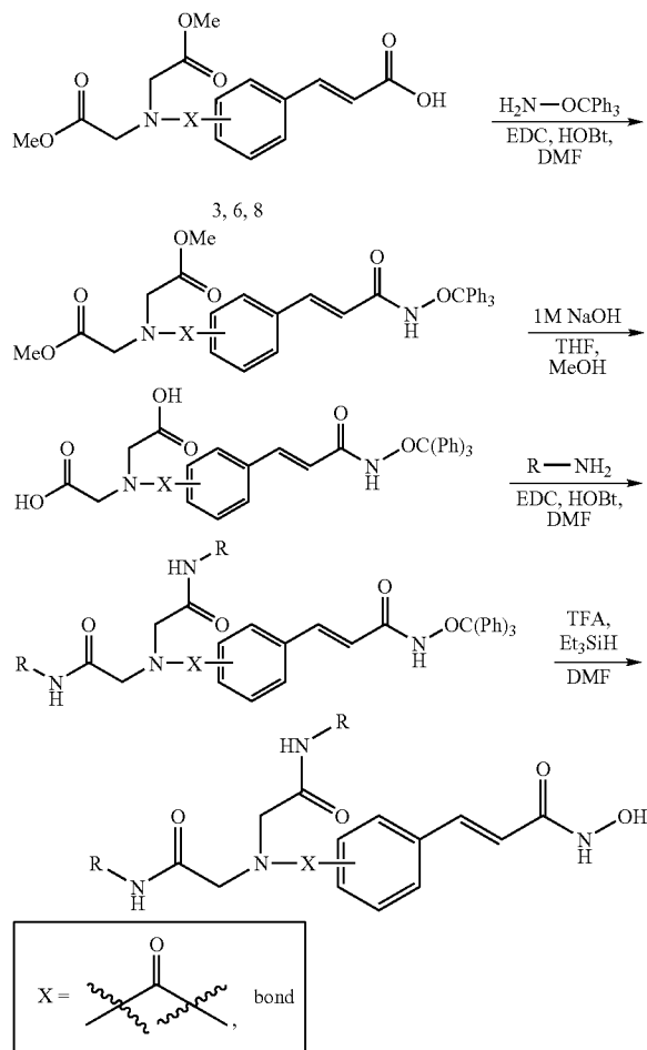
SCHEME 4
