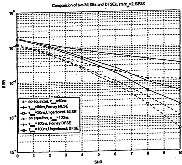
Figure 6: Comparison of two MLSEs and their DFSE, joint channel and data estimation, BPSK
