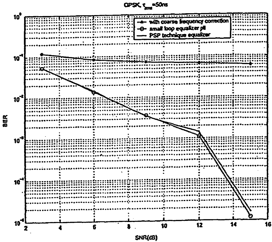
Figure 7: The BER comparison of two receiver architectures
