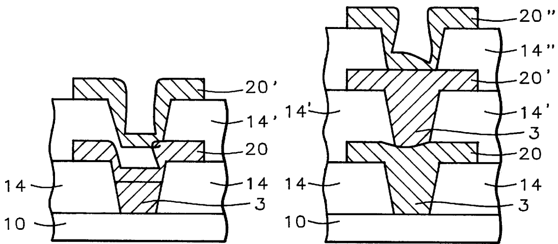
FIG. 2C - Prior Art
