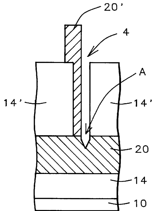
FIG. 3 - Prior Art
