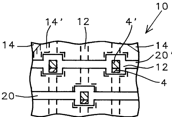
FIG. 1C - Prior Art
