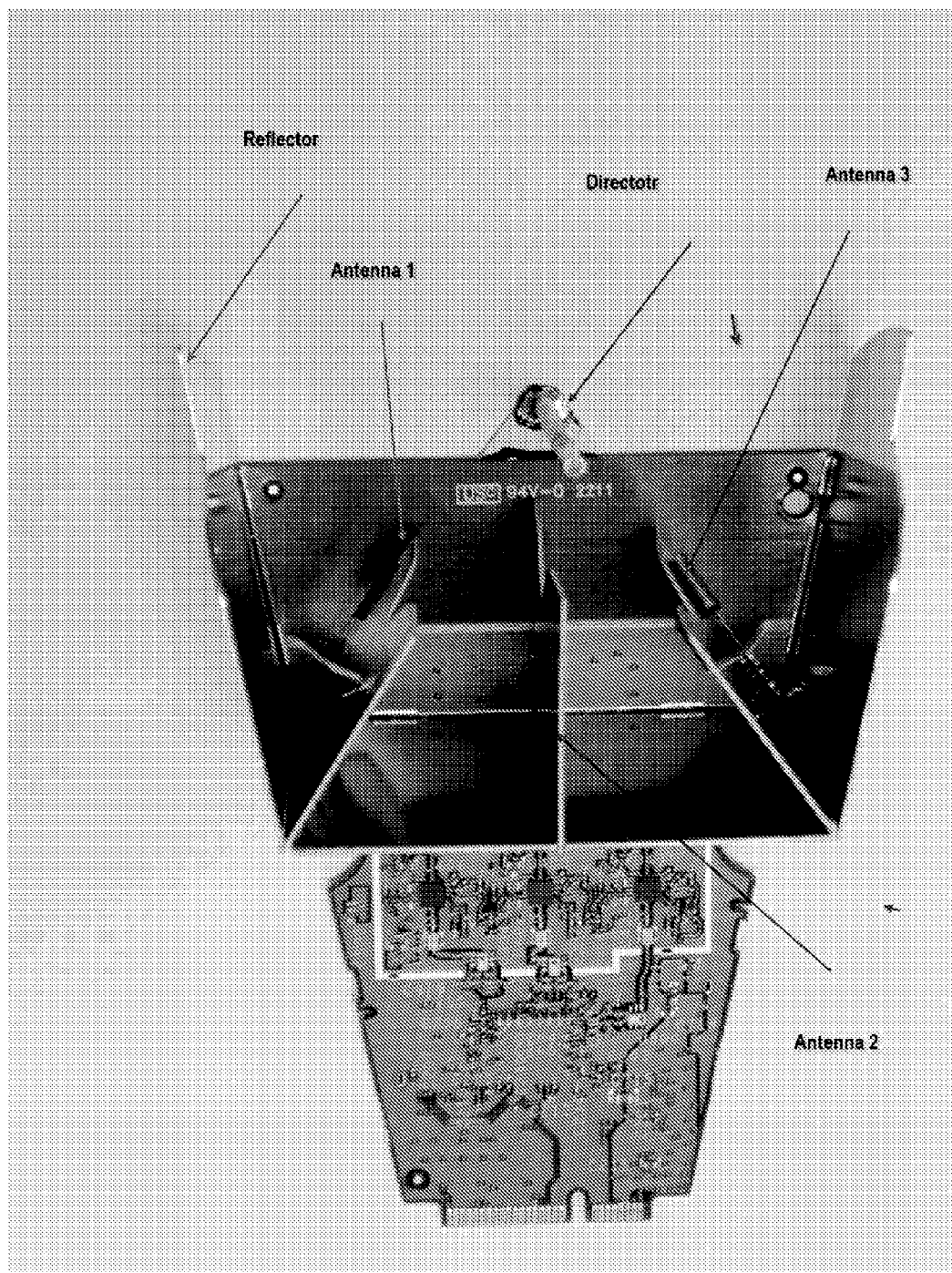
Figure 7- RF card with antennas and director, top view
